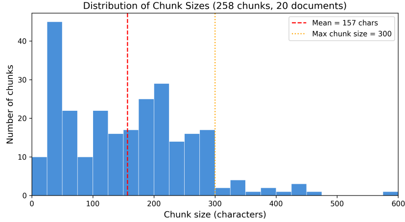
Figure 3.3: Distribution of chunk sizes across the 258-chunk Vietnamese HR corpus. Most chunks are 80–250 characters, reflecting the natural paragraph structure of Vietnamese policy documents.
