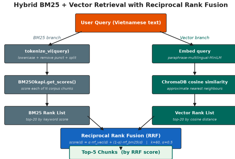
Figure 3.4: Hybrid retrieval pipeline. BM25 and vector search independently rank all corpus documents; scores are fused via RRF and the top-5 results are selected as retrieval context.
