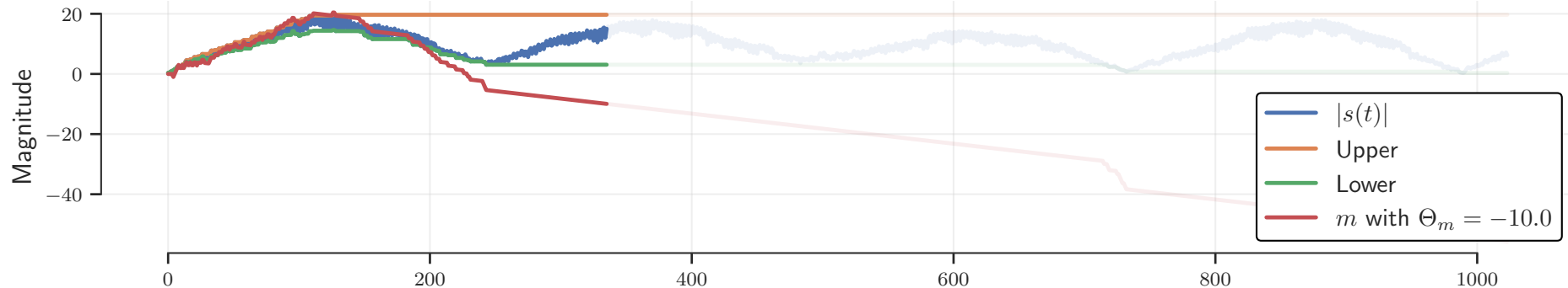
Non-resonating Neuron ( \omega_r = 10.5, \phi_v = 4.0 )
