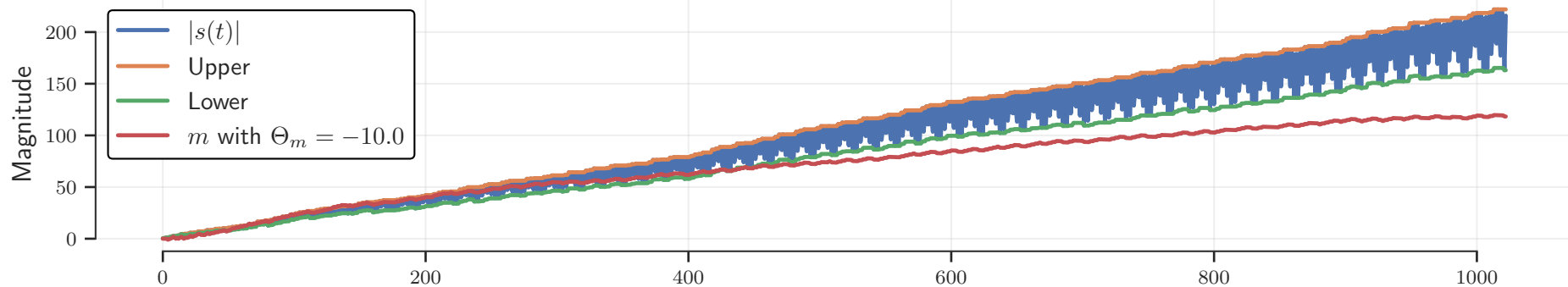
Resonating Neuron ( \omega_r = 10.0, \phi_v = 4.0 )
