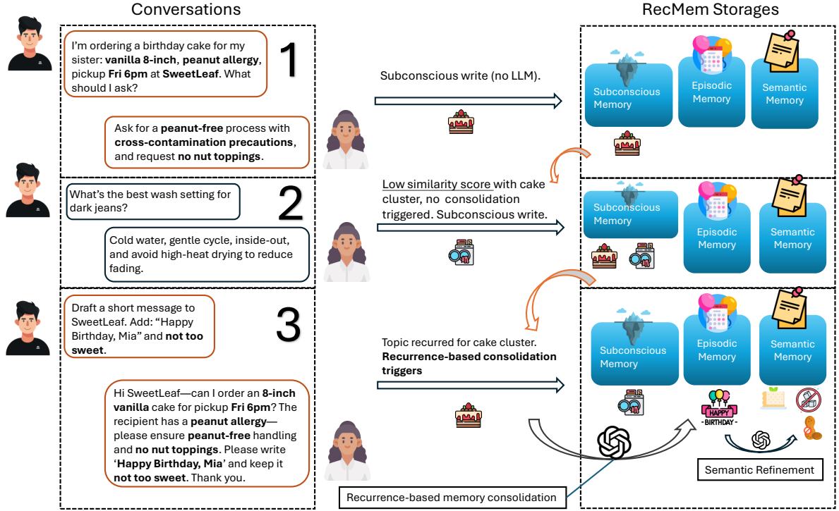
Figure 3: A simplified memory ingestion process in RecMem
