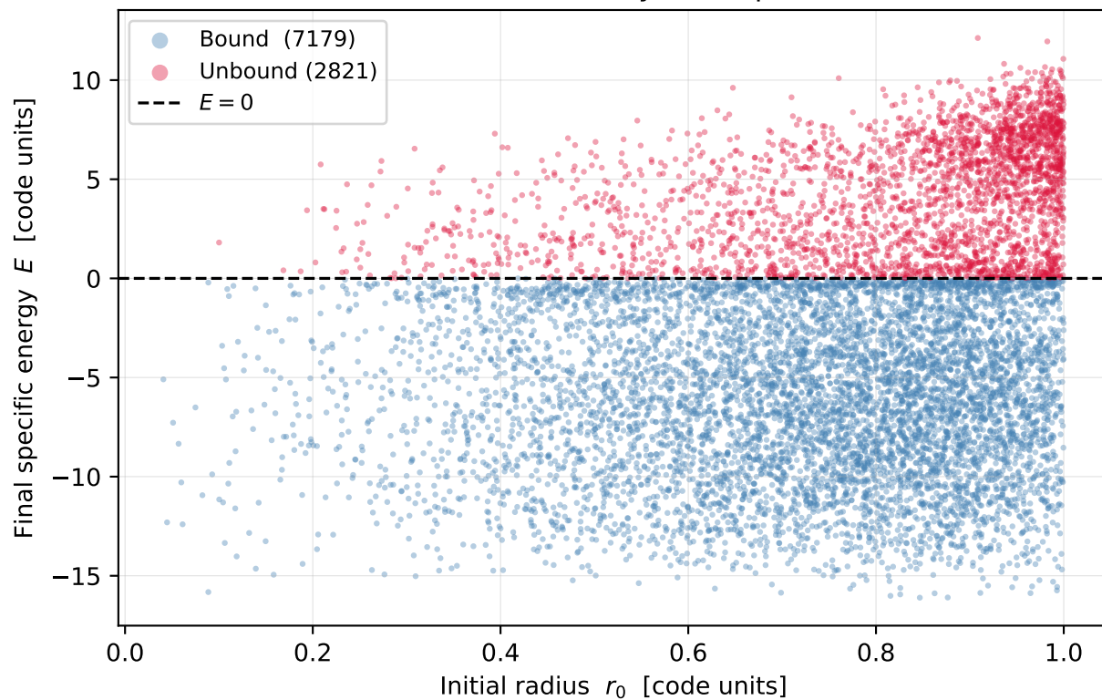
Bound / Unbound by initial position
