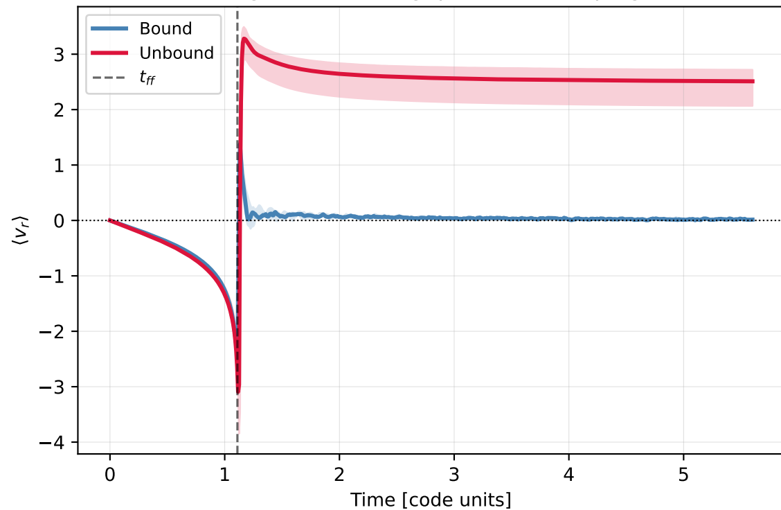
Mean radial velocity (negative=infalling, positive=escaping)
