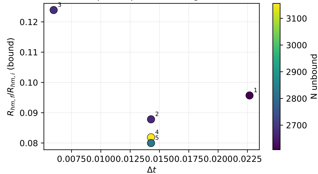
Collapse depth vs. timing offset
