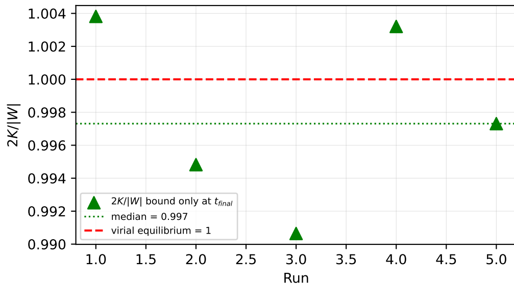
Virial ratio — bound only at t_{\text{final}}
