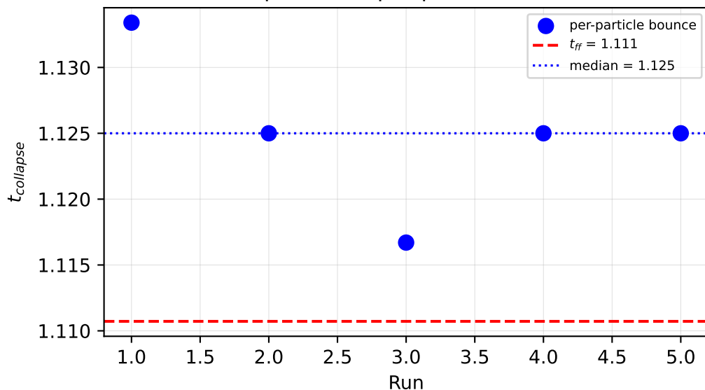
Collapse time (per-particle bounce)
