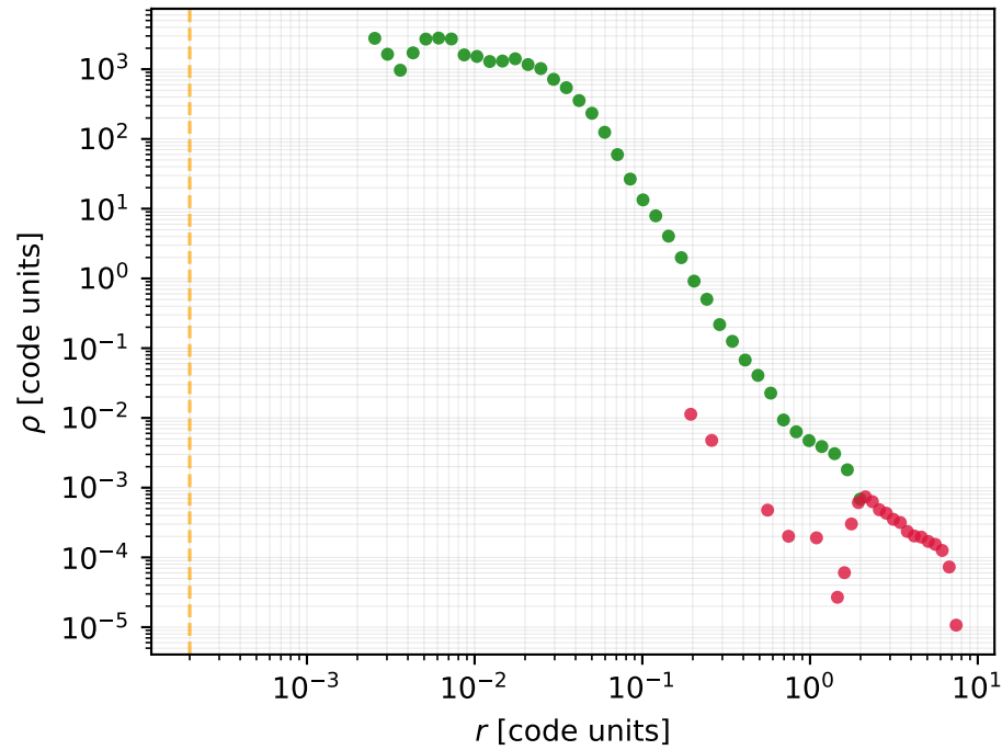
Density profile evolution — eps_0p0001 green = bound | red = unbound (both measured from bound CM) dashed = 2\varepsilon = 0.0002 (softening floor, fit cutoff)
