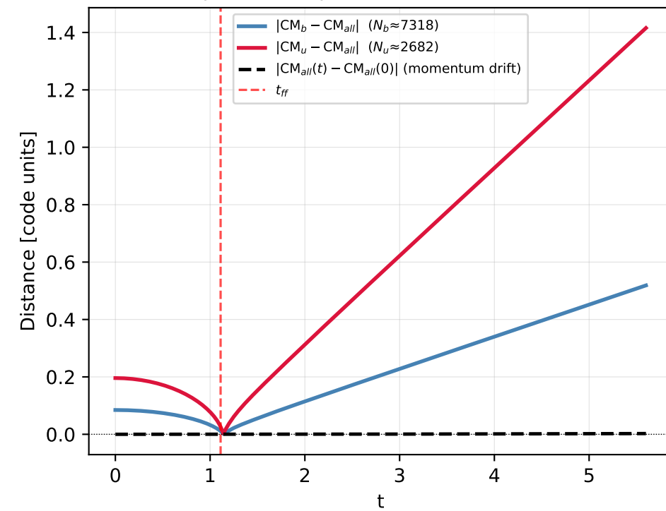
Center-of-mass tracks dashed = |CM_{all} \text{ drift}| ( \rightarrow 0 if momentum conserved)
