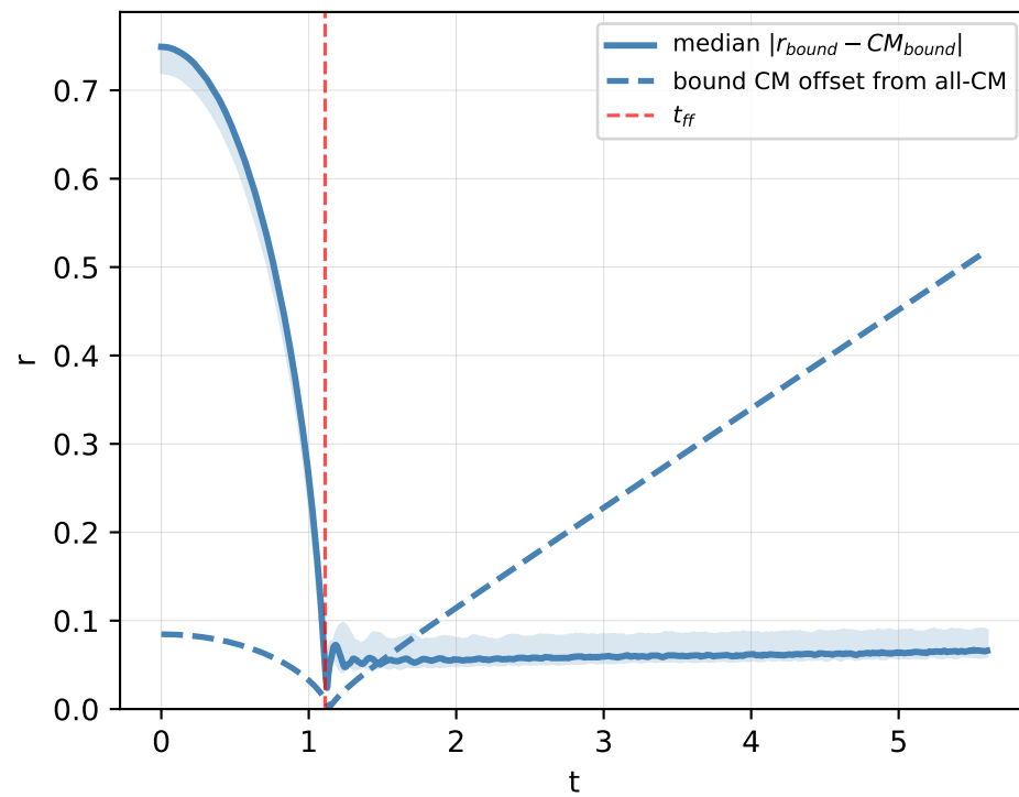
Bound particles (r from bound CM)
