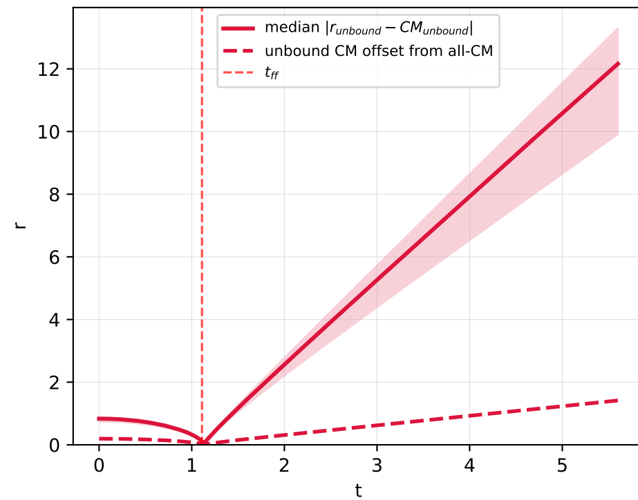
Unbound particles (r from unbound CM)
