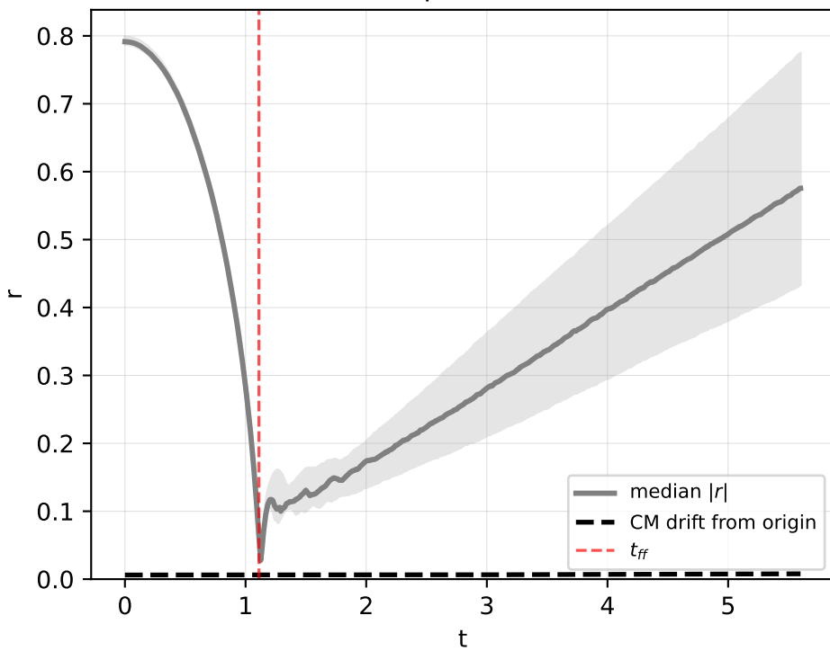
All particles
