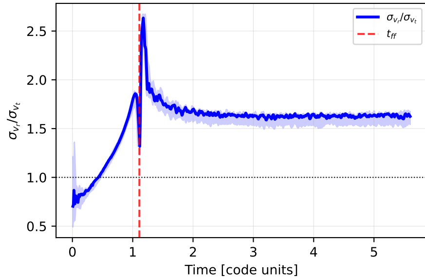
Radial/tangential dispersion ratio
