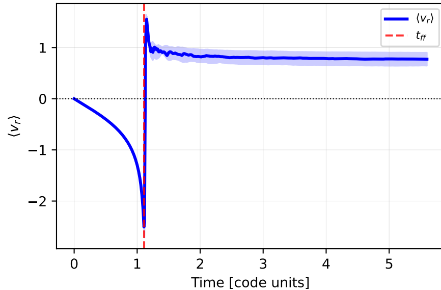
Mean radial velocity
