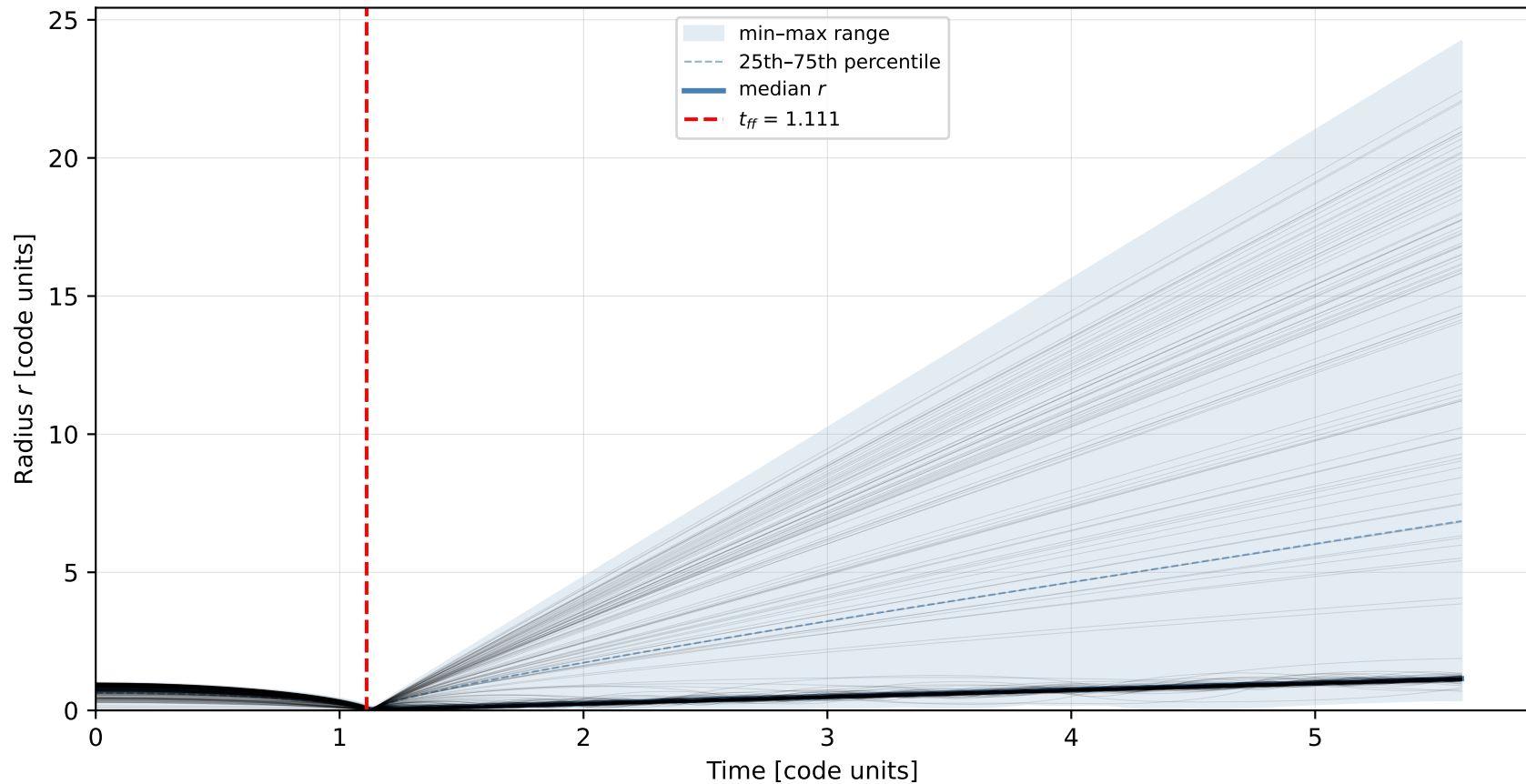
Homogeneous sphere collapse: r(t) ( N = 10000 , treecode)
