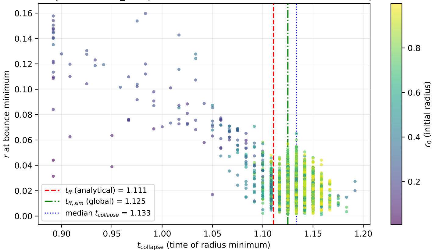
Collapse time per particle (treecode, N = 10000 , \text{min\_rising\_steps} = 2 ) [off-by-one fixed: t_{\text{collapse}} = \text{time of minimum} , not first outward step]
