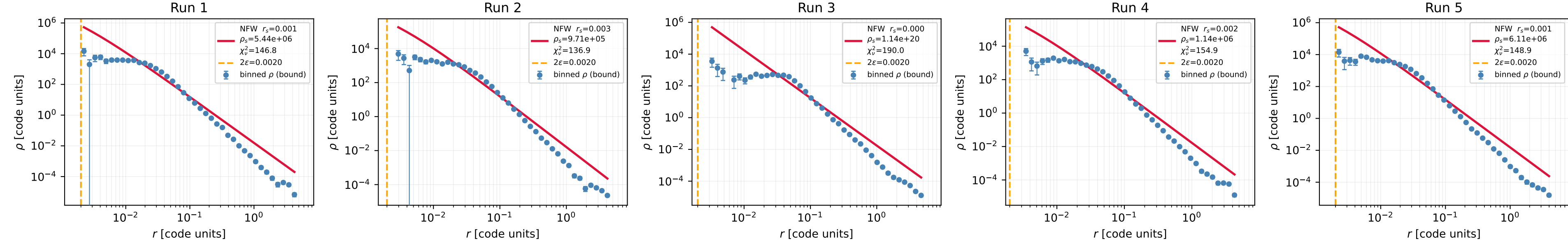
NFW density profile of bound remnant — eps_0p001 \rho(r) = \rho_s / [(r/r_s)(1 + r/r_s)^2] — fit excludes r < 2\varepsilon
