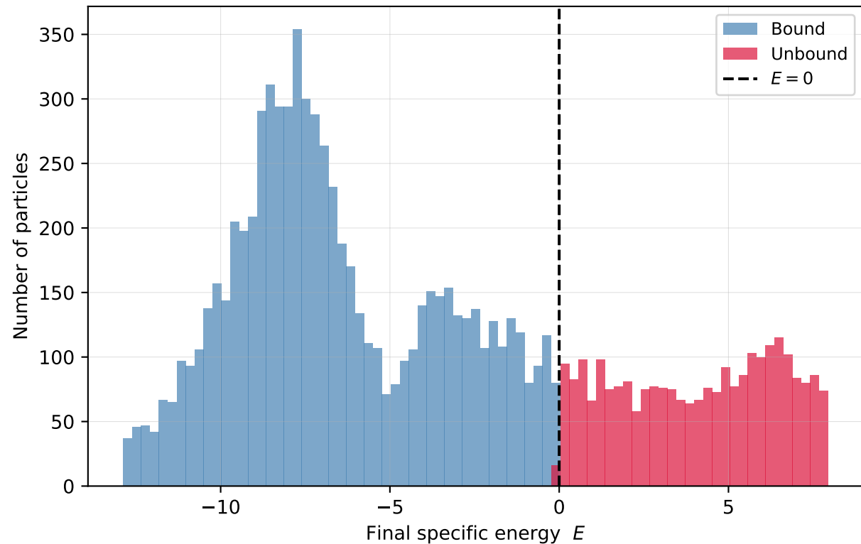
Energy distribution at final snapshot
