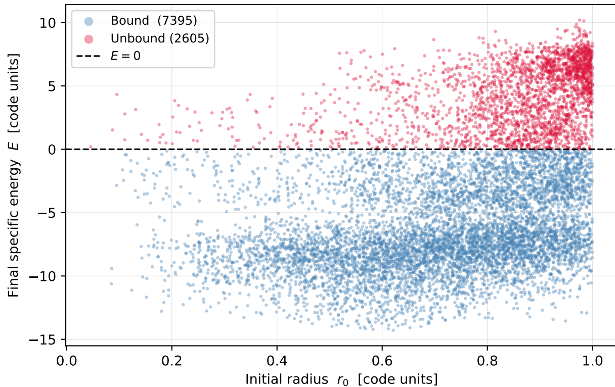
Bound / Unbound by initial position
