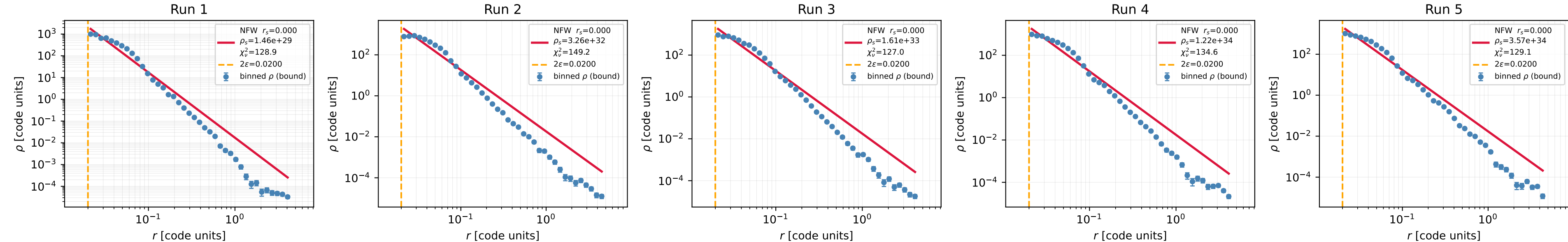
NFW density profile of bound remnant — eps_0p01 \rho(r) = \rho_s / [(r/r_s)(1 + r/r_s)^2] — fit excludes r < 2\varepsilon
