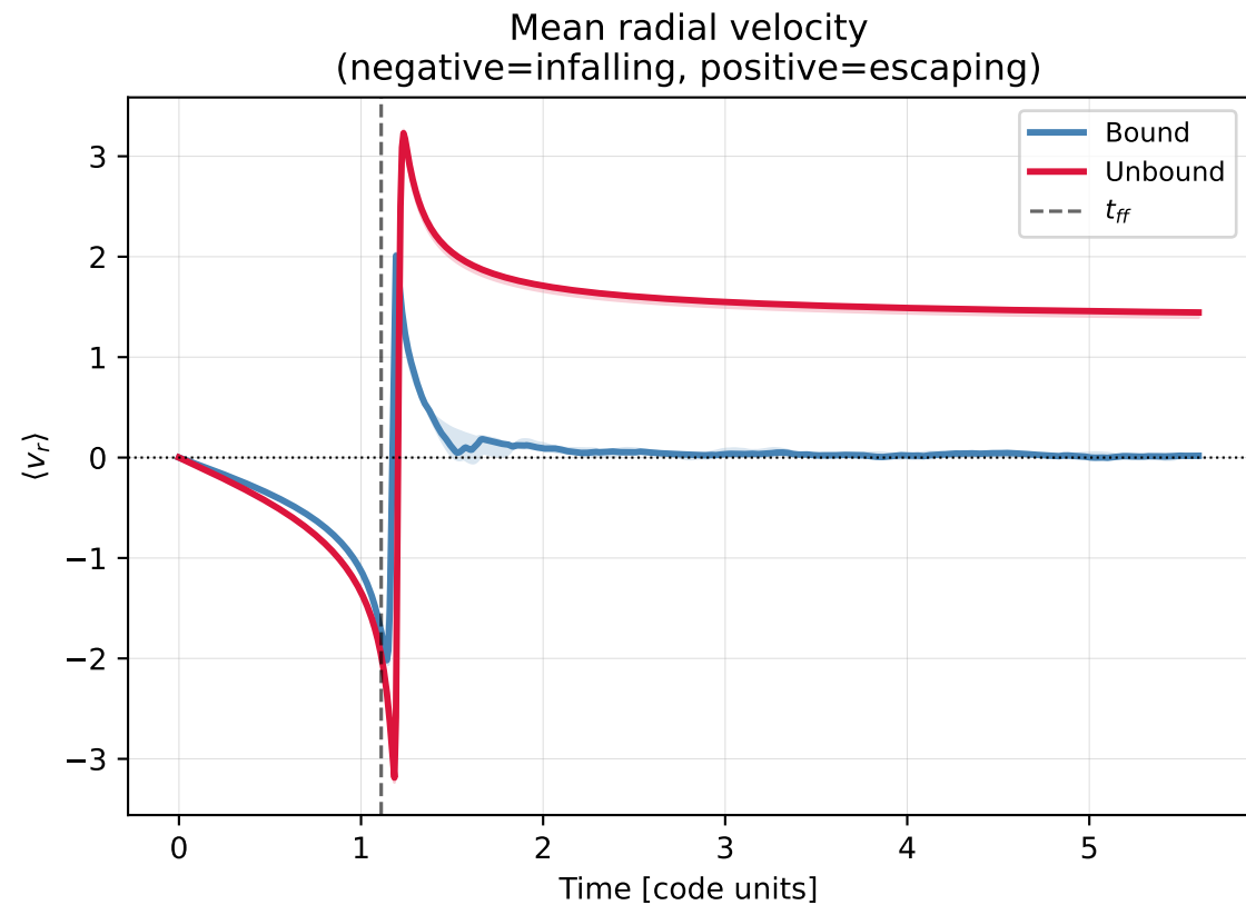
Bound vs Unbound — velocity evolution (treecode N=10000) (thick = median, shading = full range)
