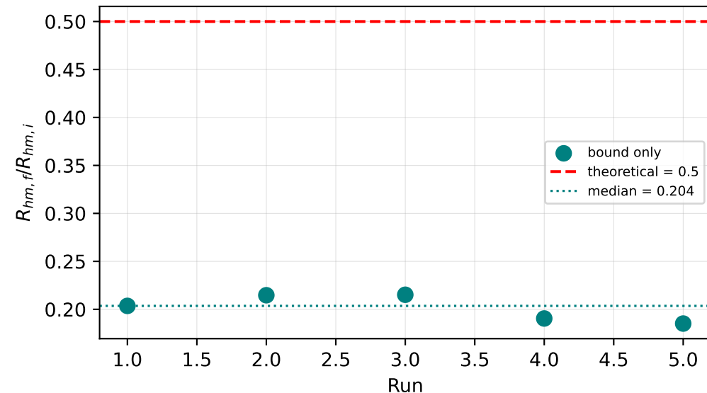
Half-mass radius ratio (bound only)
