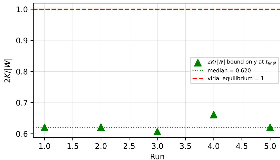
Virial ratio — bound only at t_{final}
