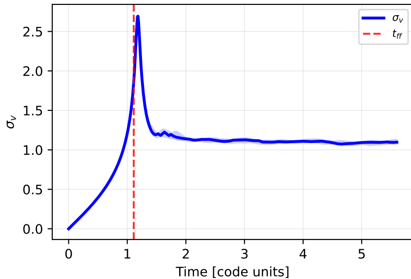
Total velocity dispersion
