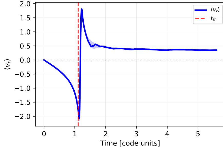
Mean radial velocity
