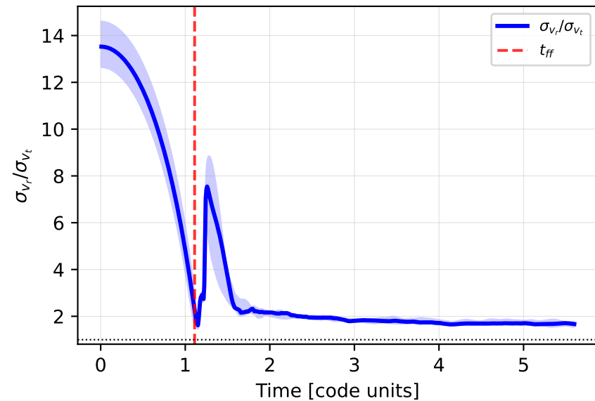
Radial/tangential dispersion ratio
