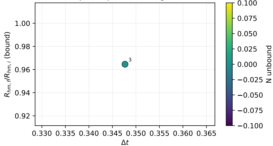
Collapse depth vs. timing offset
