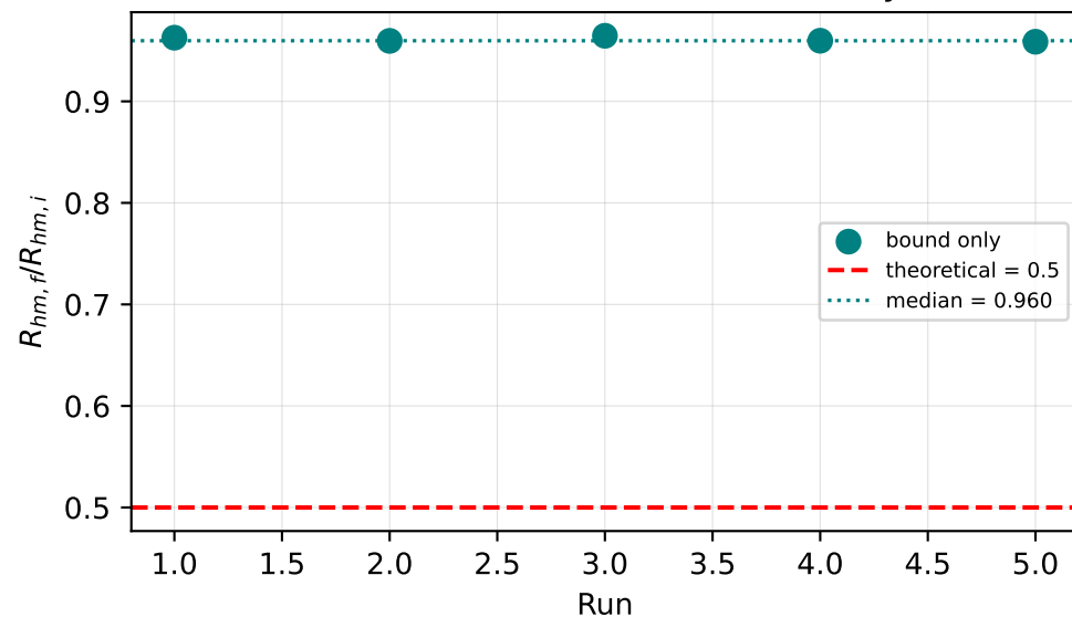
Half-mass radius ratio (bound only)
