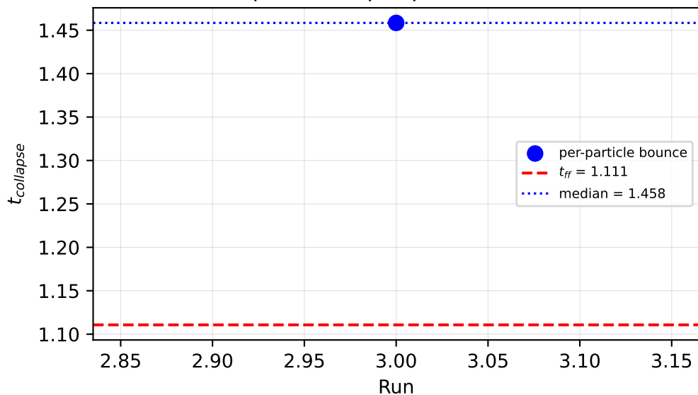
Collapse time (per-particle bounce)
