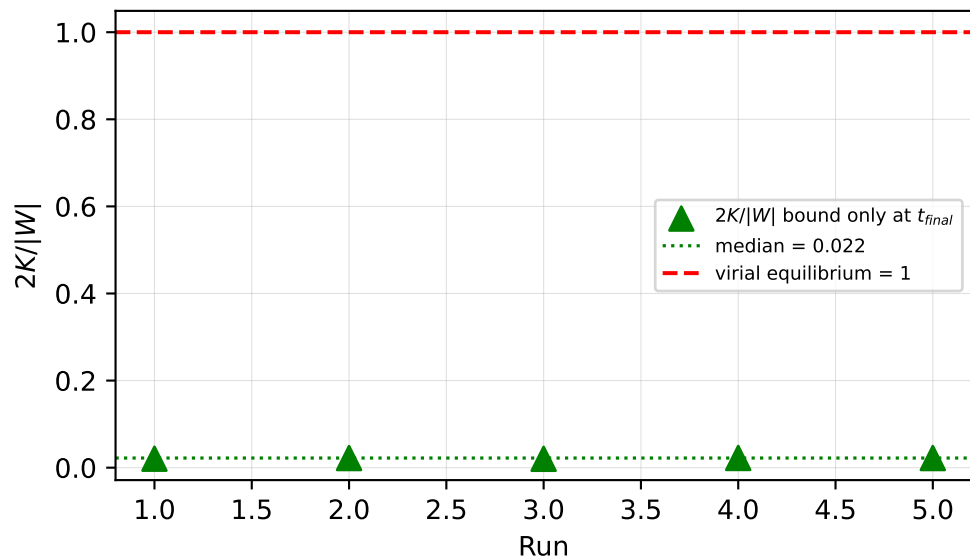
Virial ratio — bound only at t_{\text{final}}
