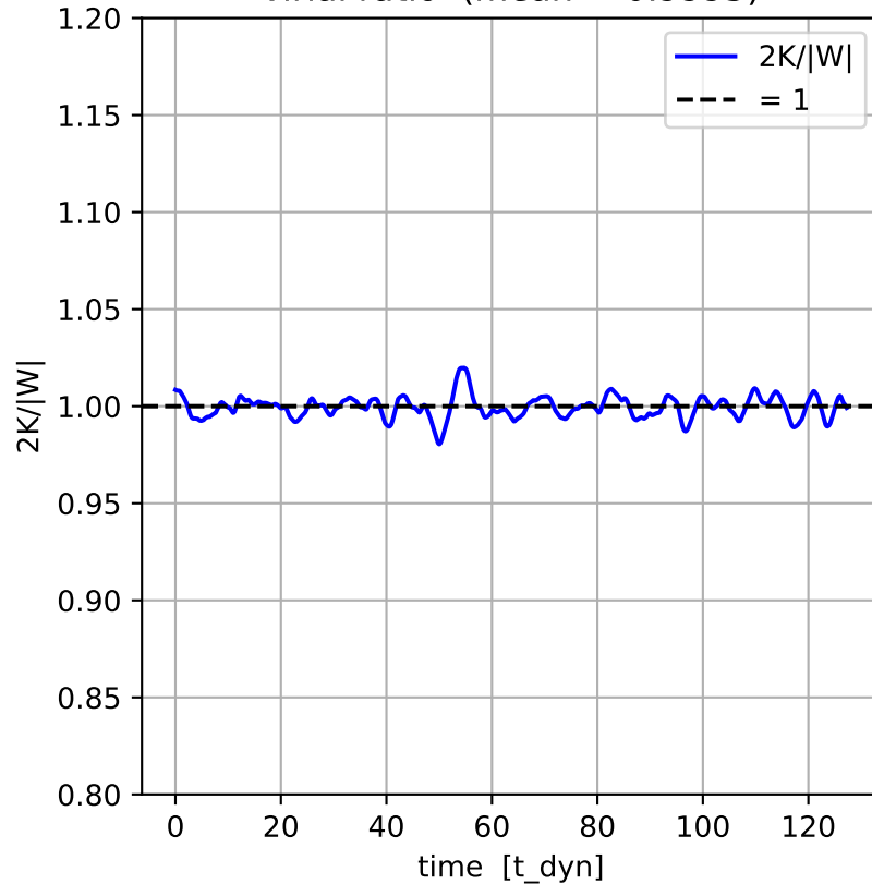
virial ratio (mean = 0.9995)
