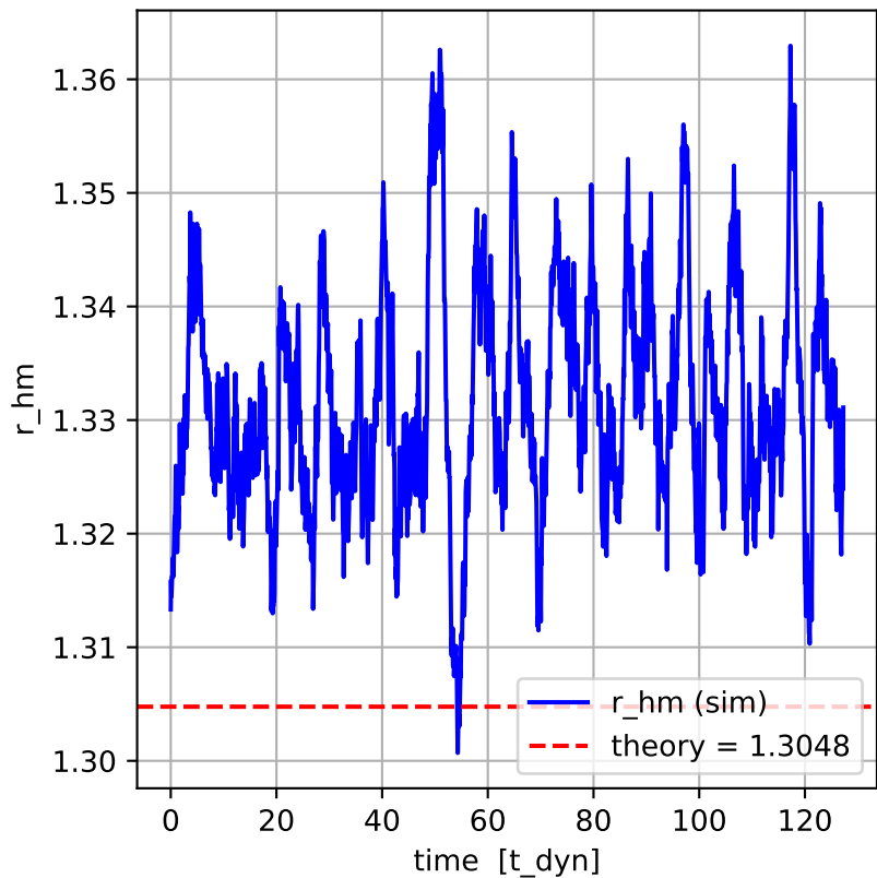
half-mass radius (drift = 1.35%)
