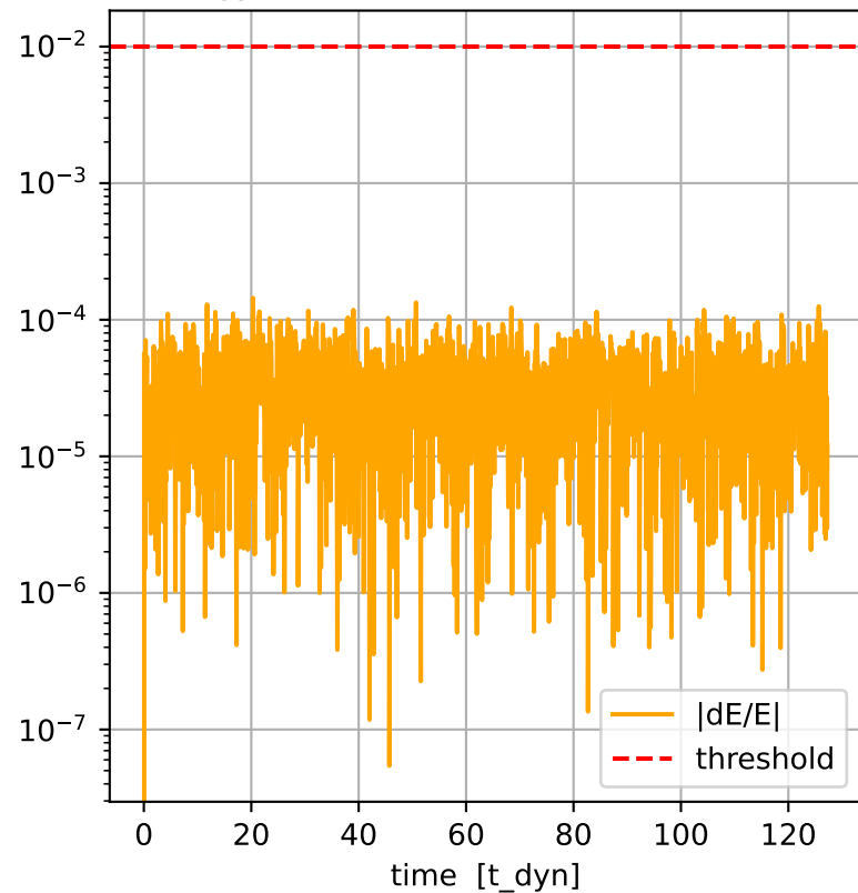
energy conservation (max = 1.44e-04)
