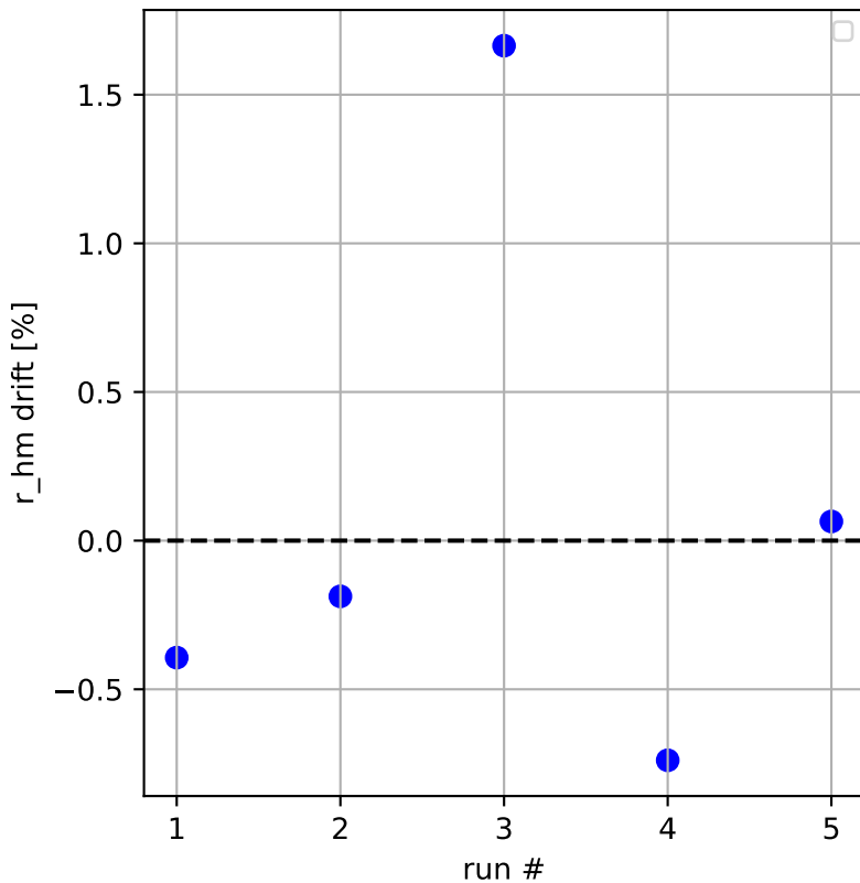
half-mass radius drift (0% = stable)
