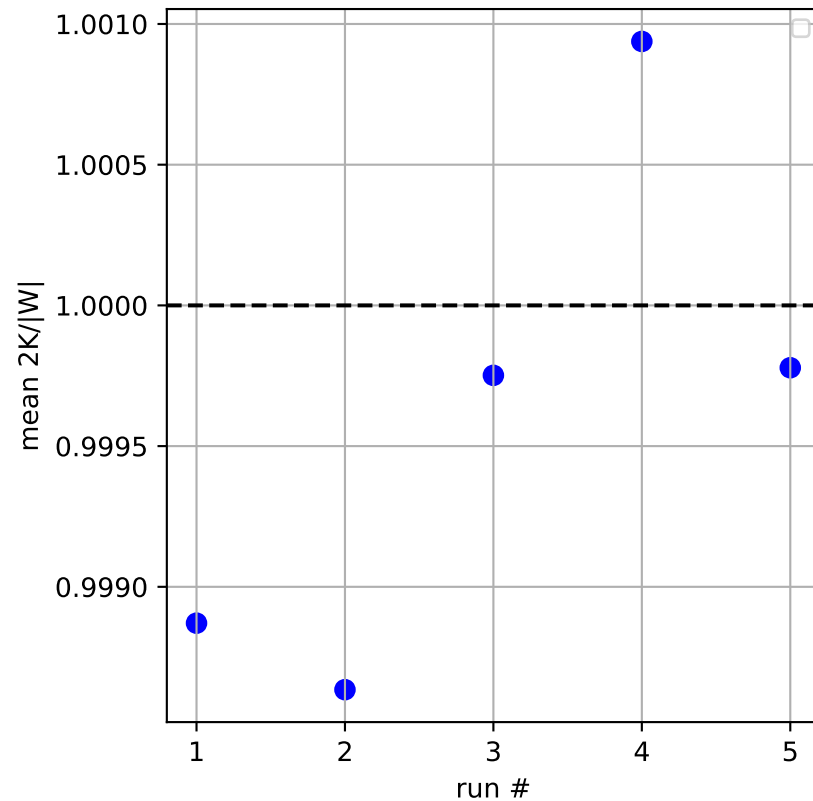
time-avg virial ratio (= 1)
