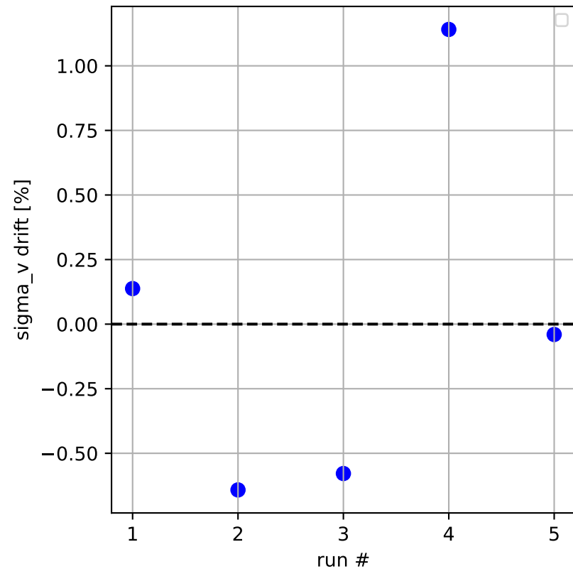
velocity dispersion drift (0% = ok)
