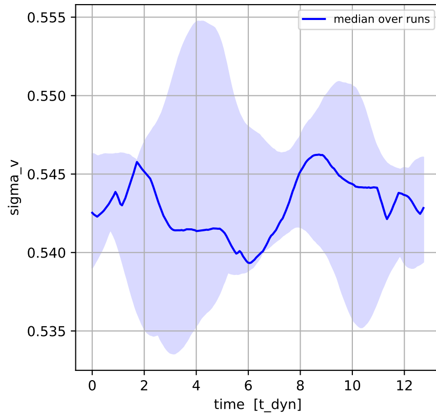
velocity dispersion
