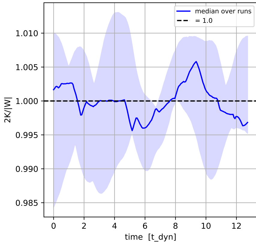
virial ratio (= 1)
