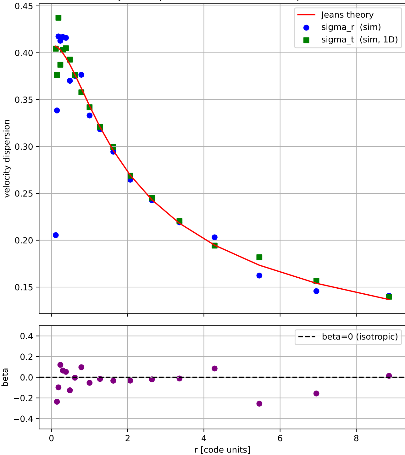
Jeans equation check — Plummer sphere
