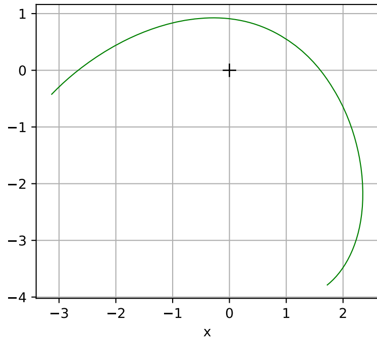
halo r \sim 3.5
