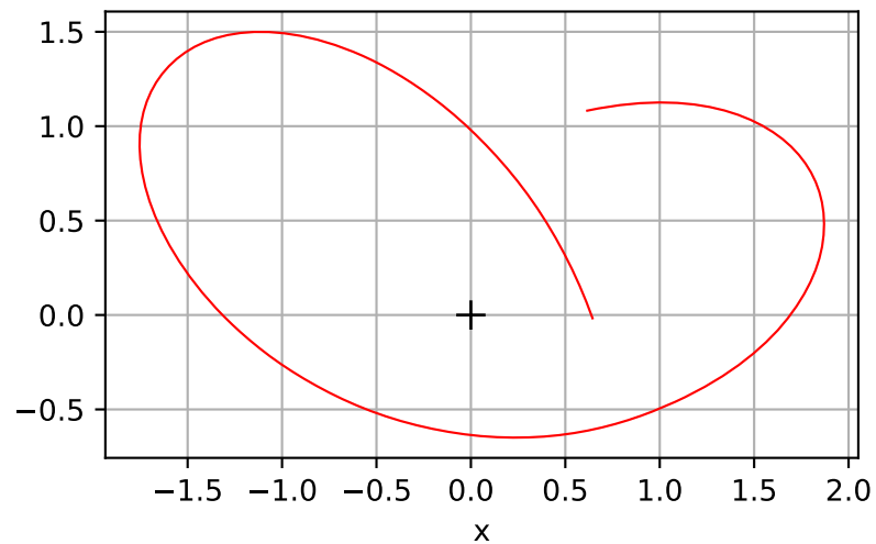
half-mass r \sim 1.3
