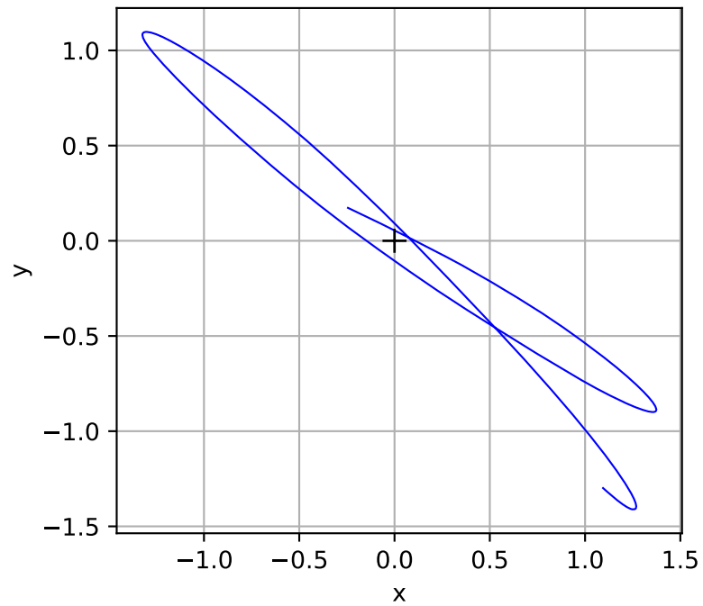
core r \sim 0.3
