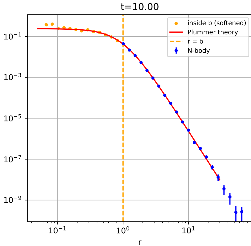
Density profile vs Plummer theory ( b=1.0 , dashed = softening r=b )
