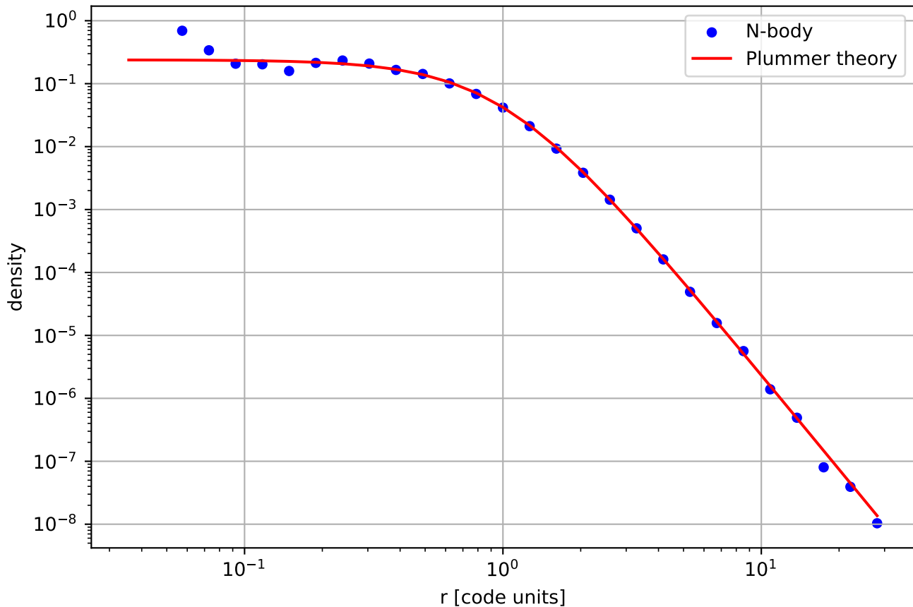
Density profile vs Plummer (m=5 polytrope)
