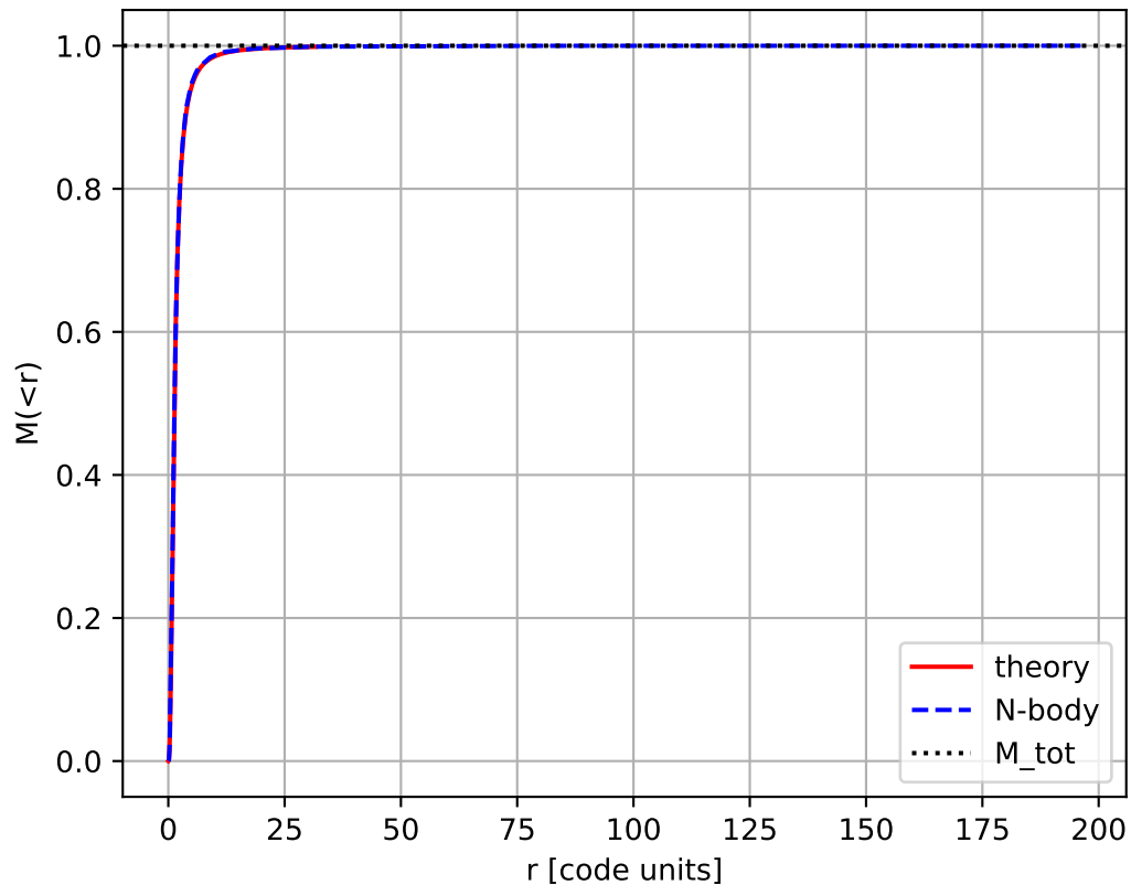
cumulative mass
