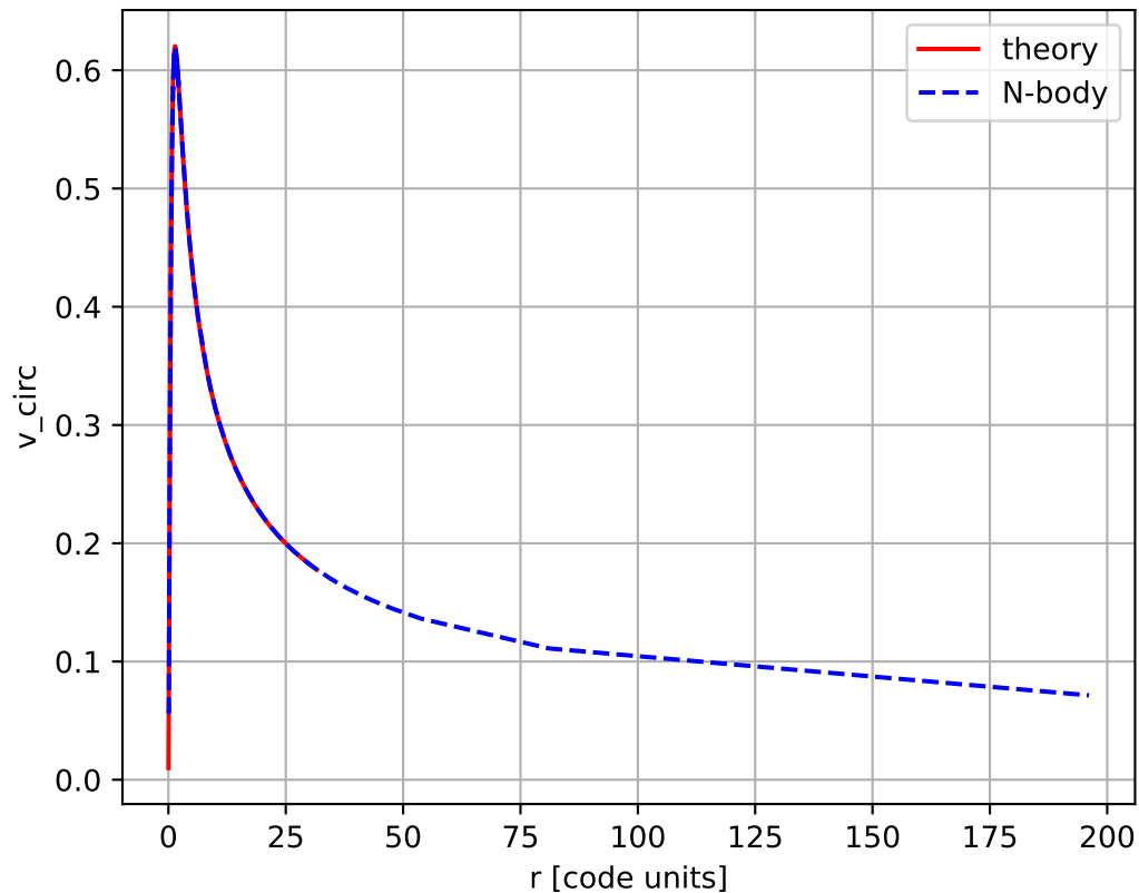
circular velocity
