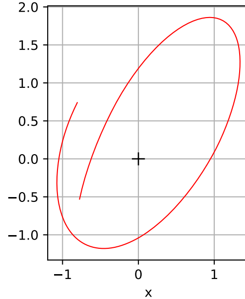
half-mass r \sim 1.3
