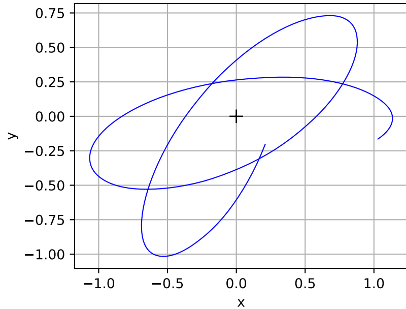
core r \sim 0.3
