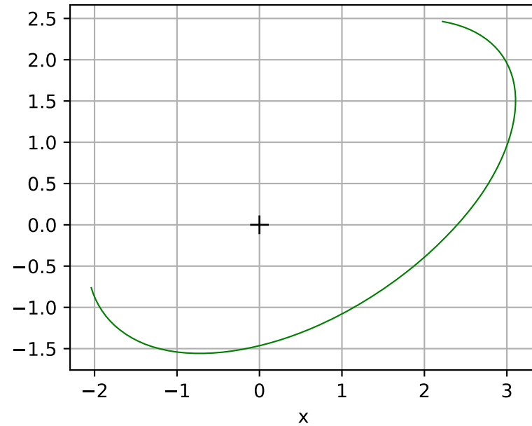
halo r \sim 3.5
