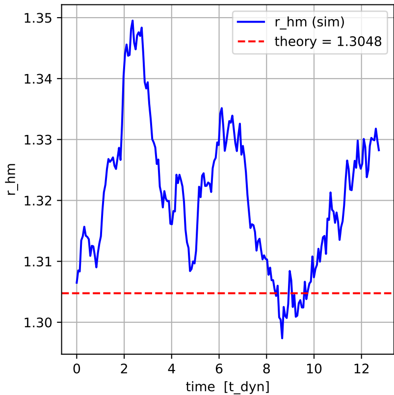
half-mass radius (drift = 1.66%)
