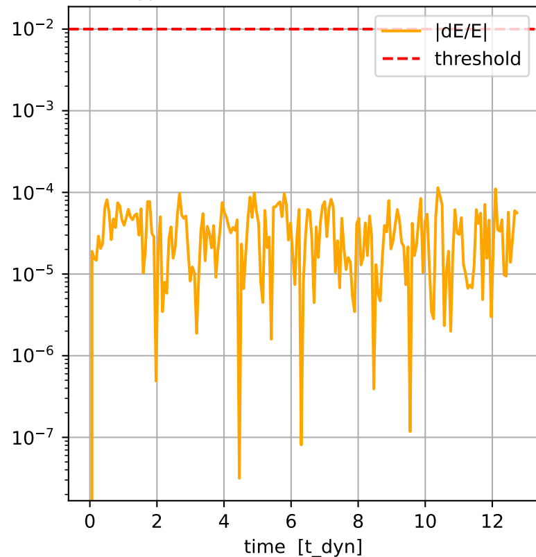
energy conservation (max = 1.14e-04)
