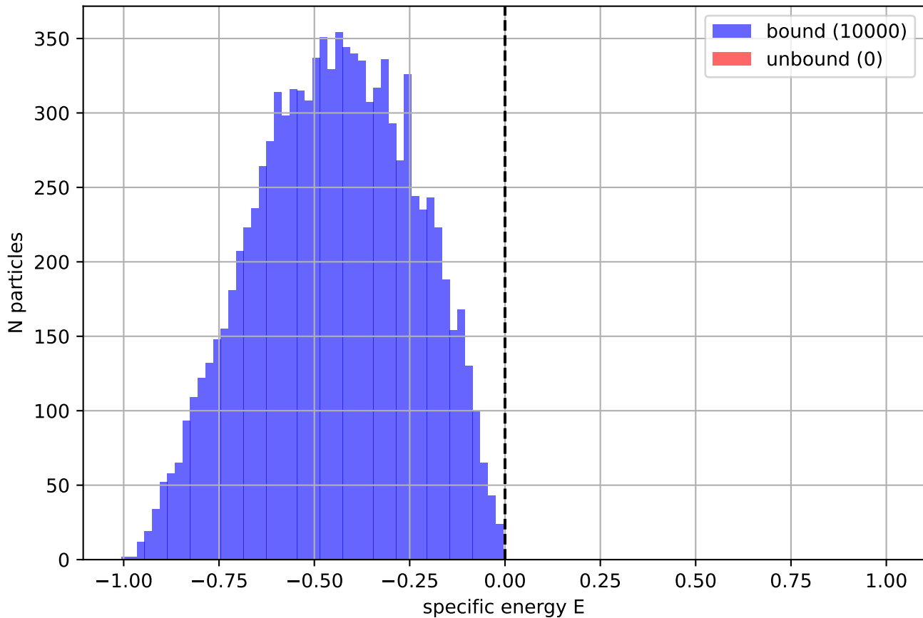
Energy distribution at final snapshot
