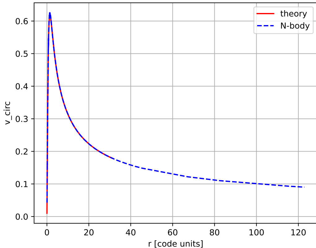
circular velocity
