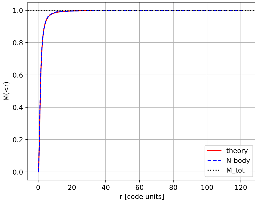
cumulative mass
