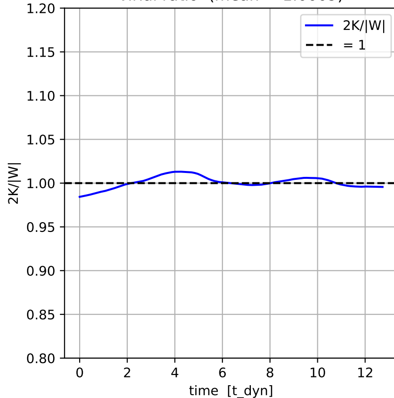
virial ratio (mean = 1.0009)
