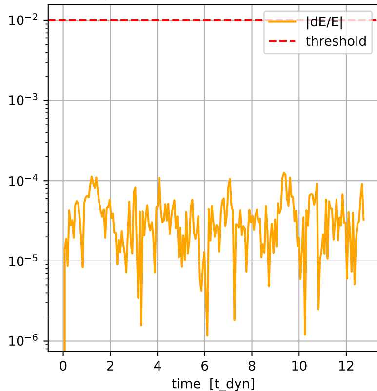
energy conservation (max = 1.25e-04)
