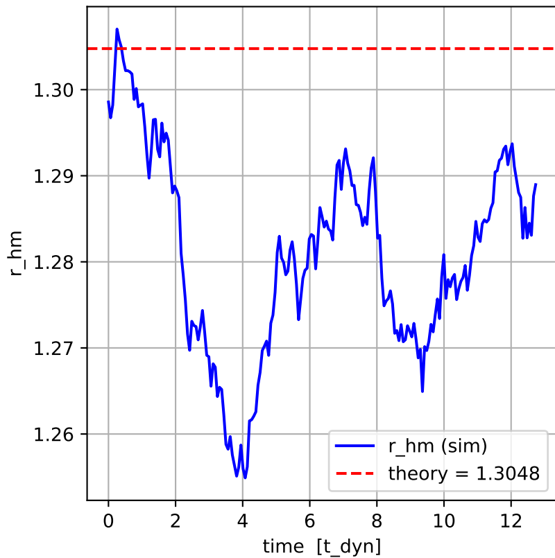
half-mass radius (drift = -0.74%)
