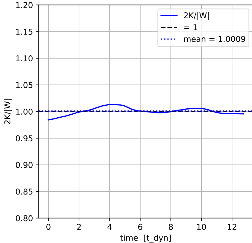
virial ratio
