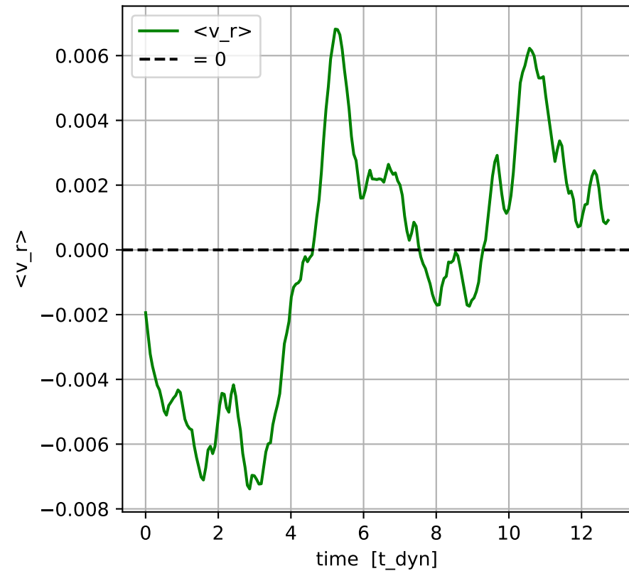
mean radial velocity (should be ~0)
