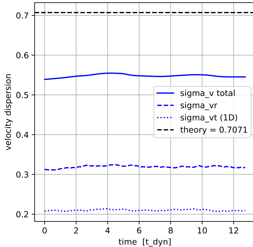
velocity dispersion
