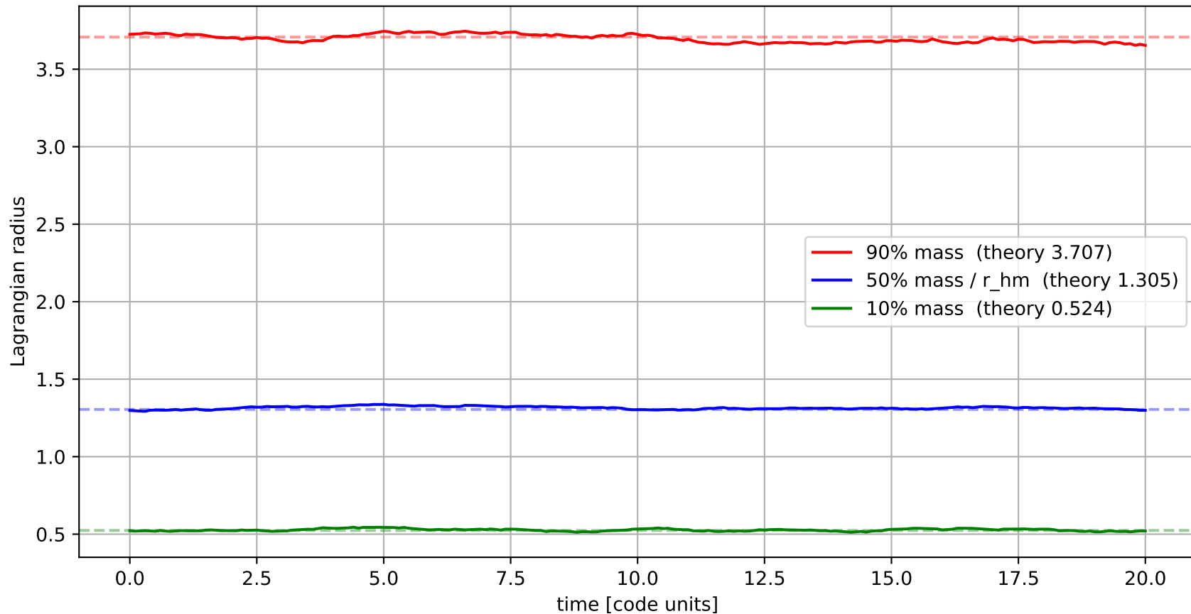
Lagrangian radii vs time (should be flat)
