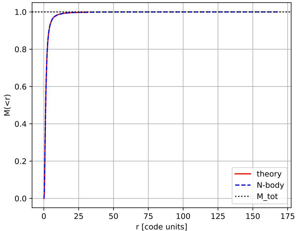
cumulative mass
