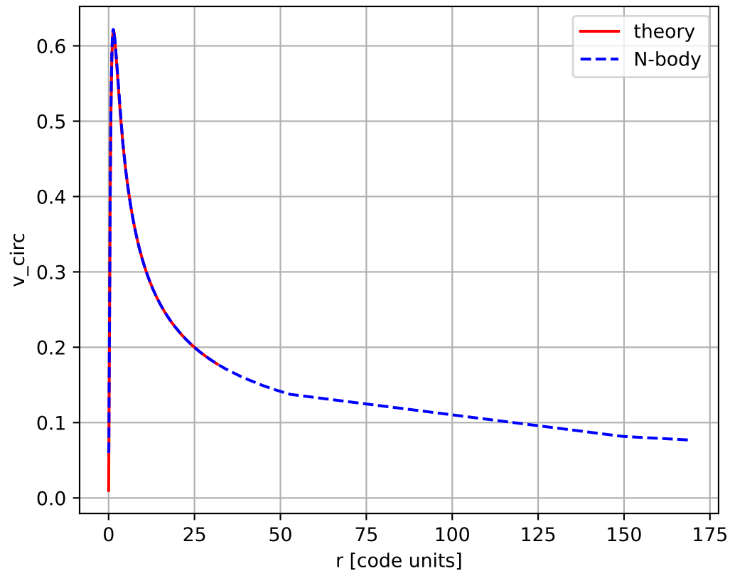
circular velocity
