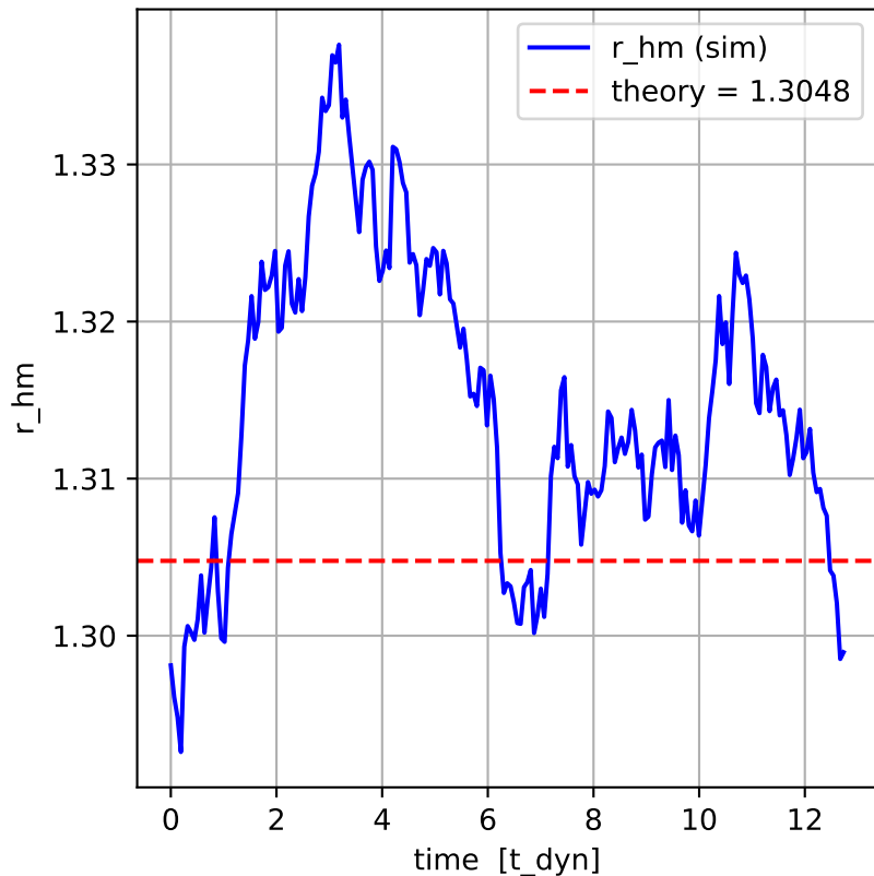
half-mass radius (drift = 0.06%)
