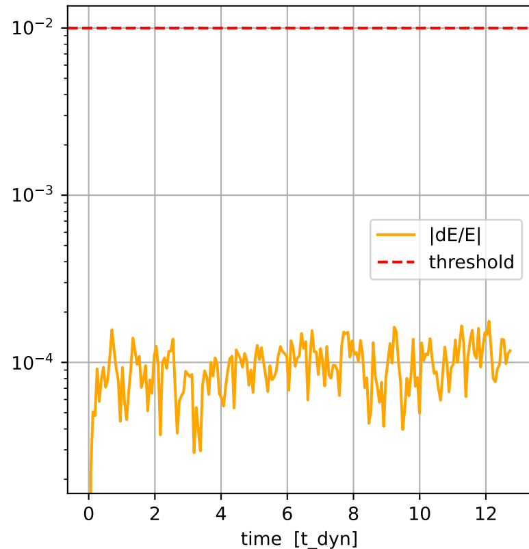
energy conservation (max = 1.76e-04)
