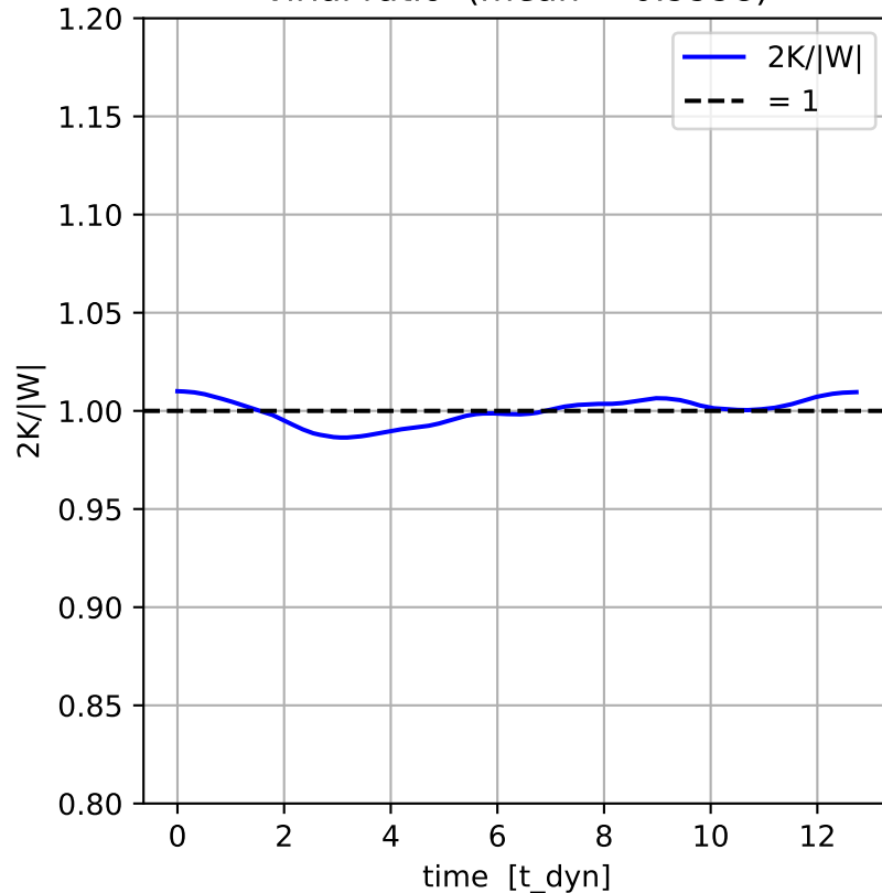
virial ratio (mean = 0.9998)
