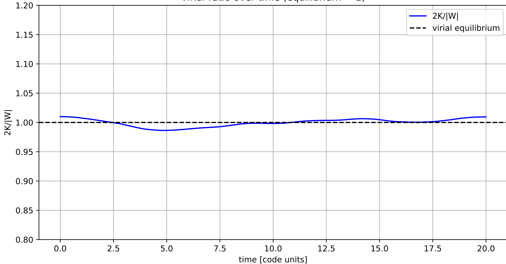
Virial ratio over time (equilibrium = 1)
