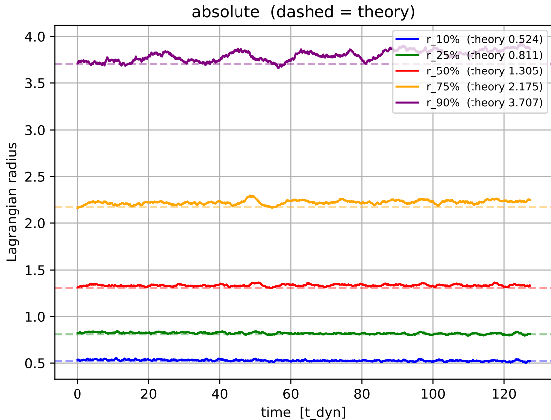
Lagrangian radii vs time (N=10000, b=1.0, eps=0.012)
