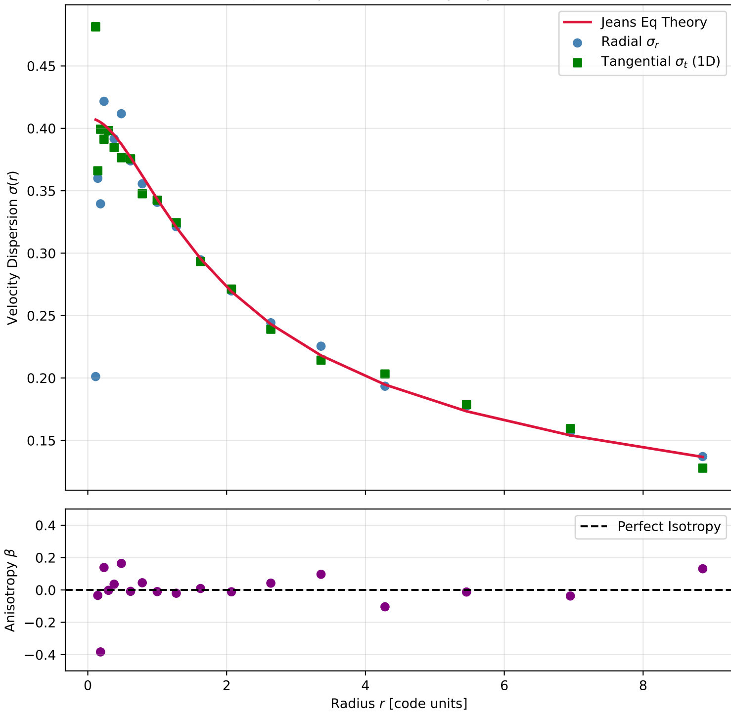
Jeans Equation & Velocity Dispersion
