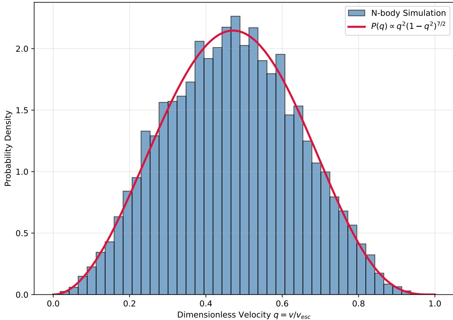
Phase-Space Velocity Distribution (Rejection Method Proof)
