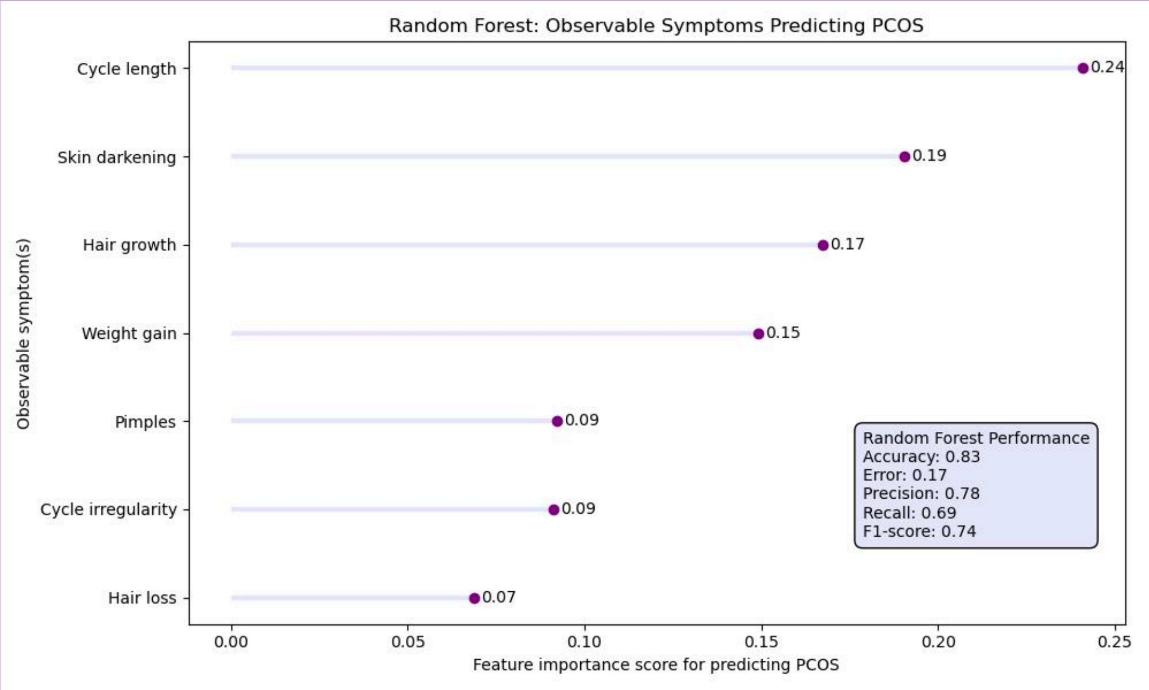
Random Forest
