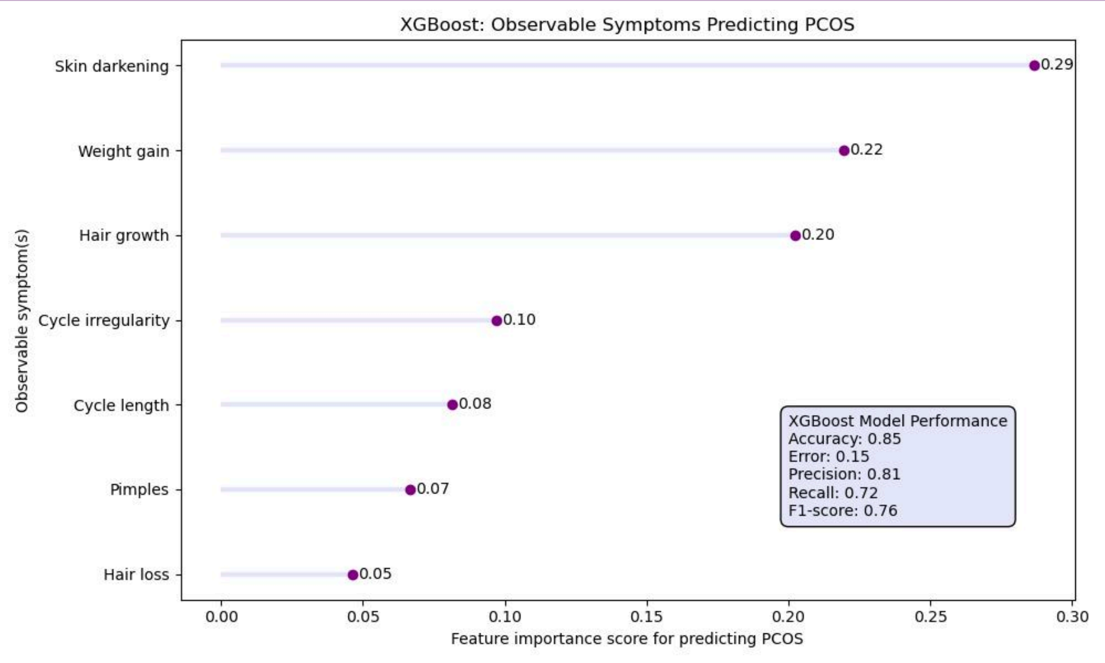
XGBoost
