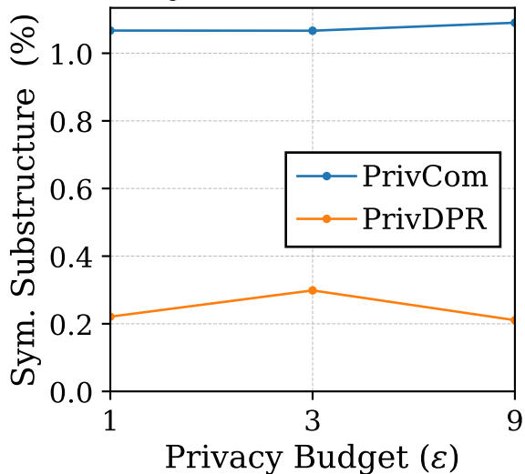
Sym. Substructure
