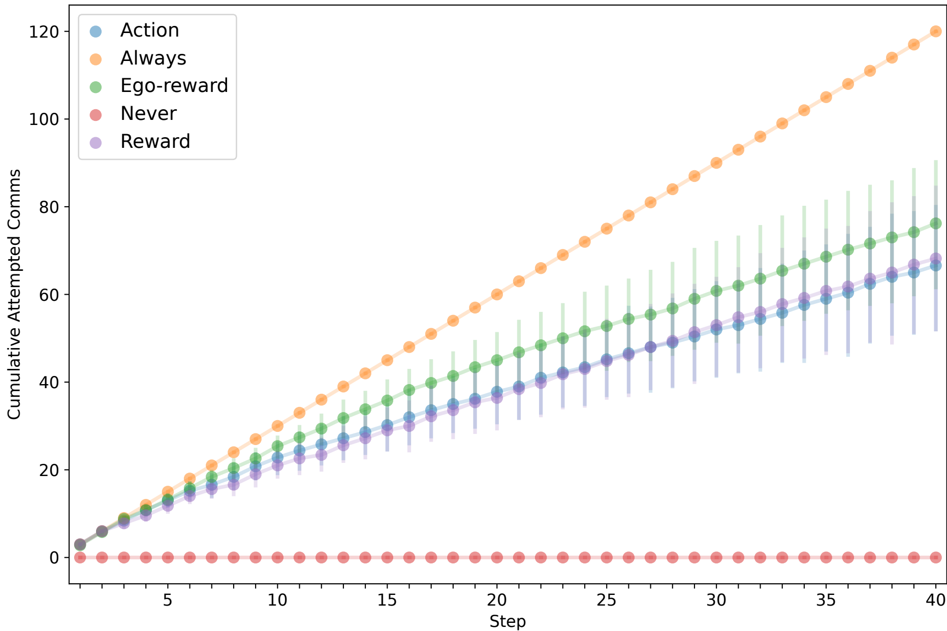
Cumulative network load over time
