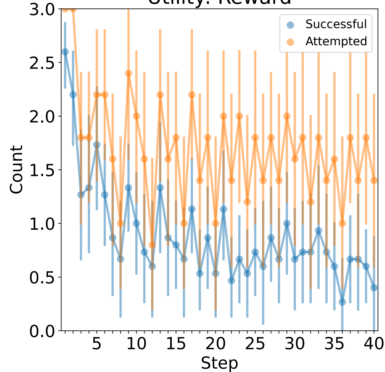
Utility: Reward
