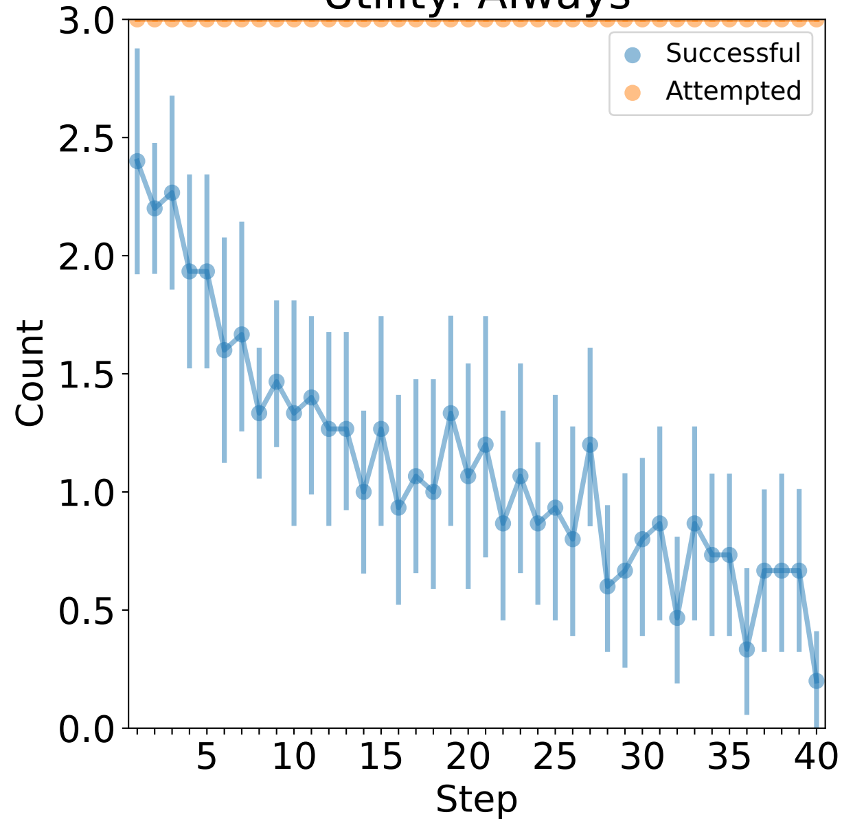
Utility: Always
