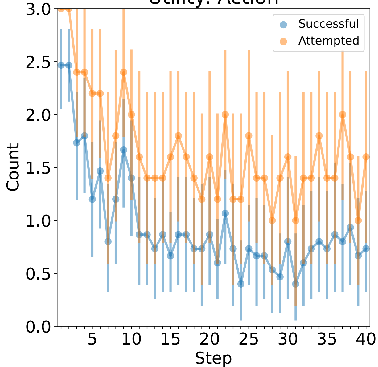
Utility: Action
