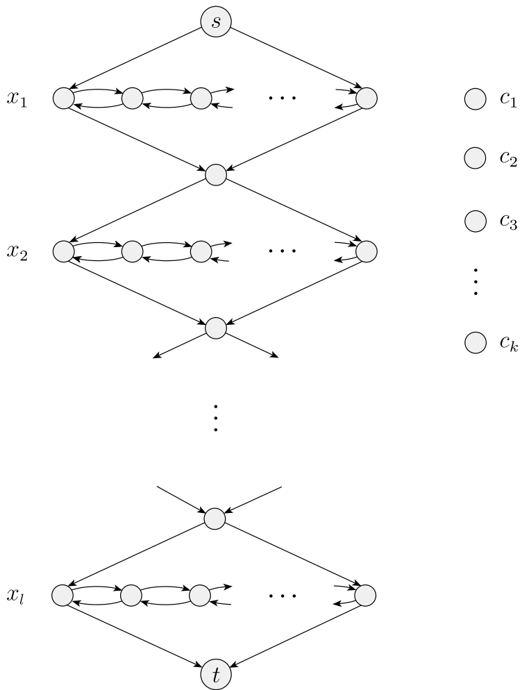
FIGURE 7.49 The high-level structure of G
