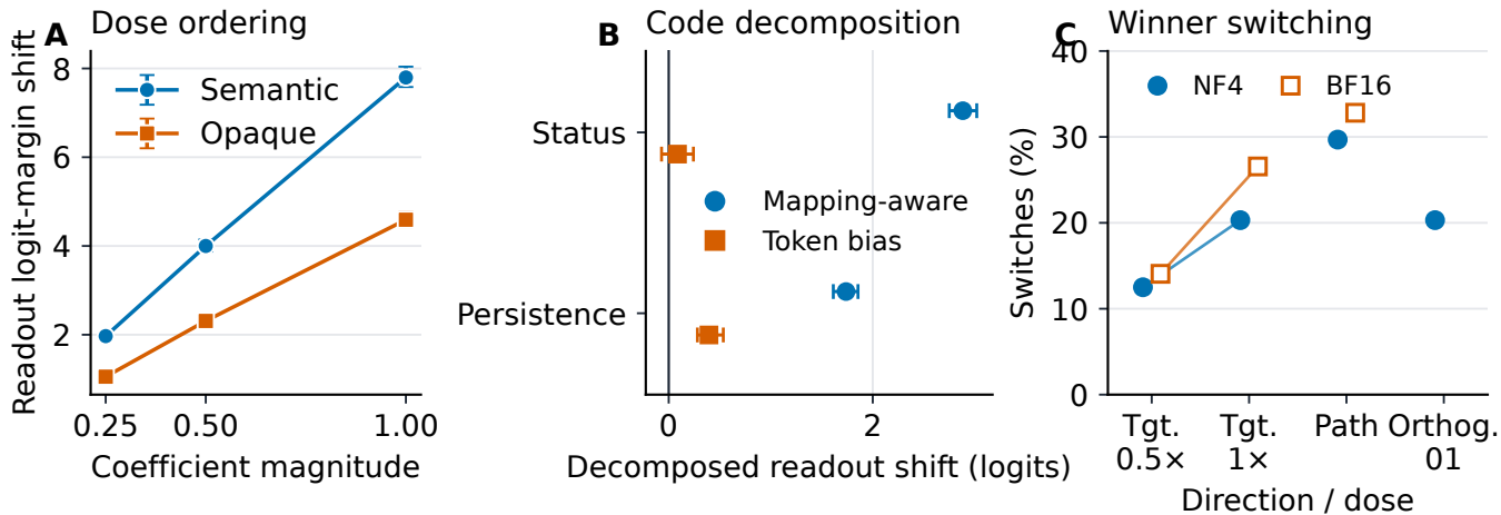
Panels A-B: lexical-frame means and 95% bootstrap intervals; panel C: exact 64-case rates (no interval).
