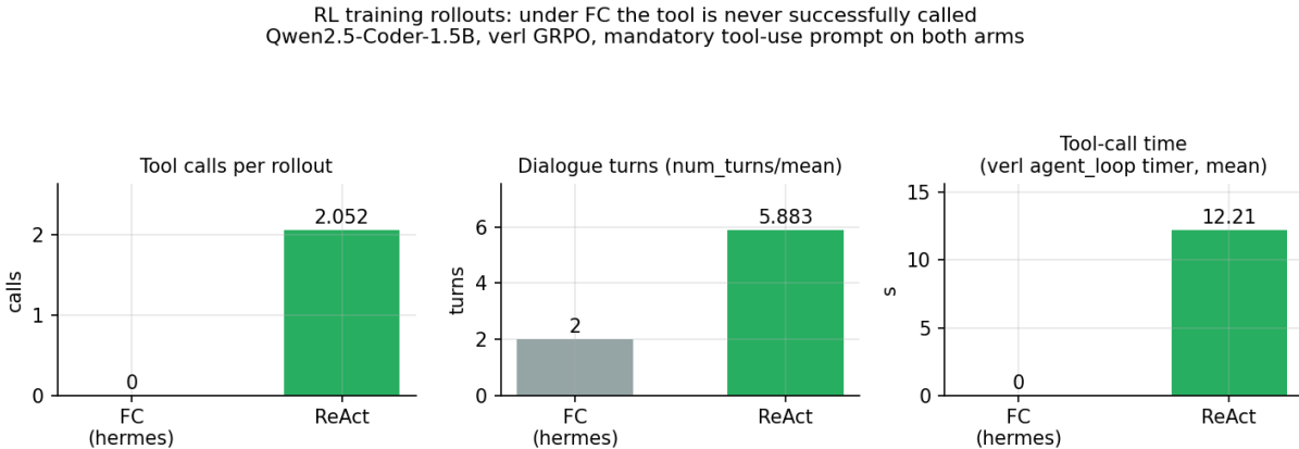
Figure 5: RL training rollouts. Under function calling the tool is never successfully called; num_turns stays pinned at its minimum of 2 and tool time is exactly zero. Prompt strength is matched across arms (both mandatory); step counts are not (10 vs 3).
