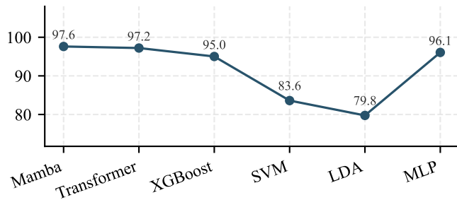
Recall
