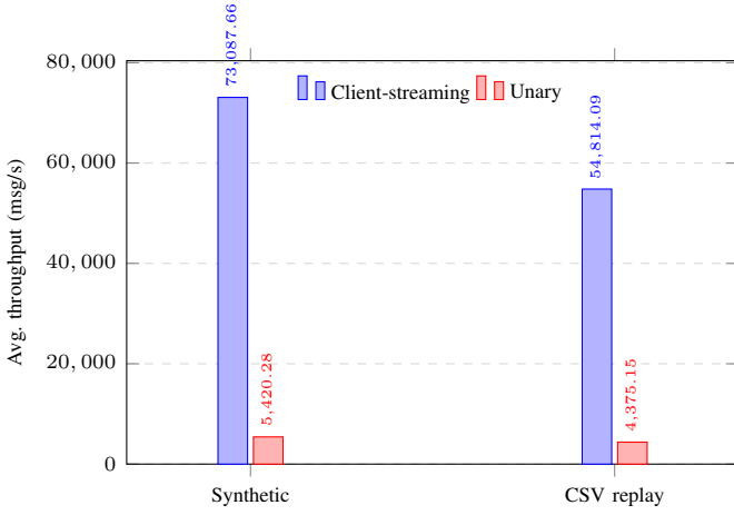
Figure 2. Average throughput for the preliminary gRPC baseline, split by workload family and transport mode. Client-streaming sustains substantially higher throughput than unary gRPC in both workload families.
