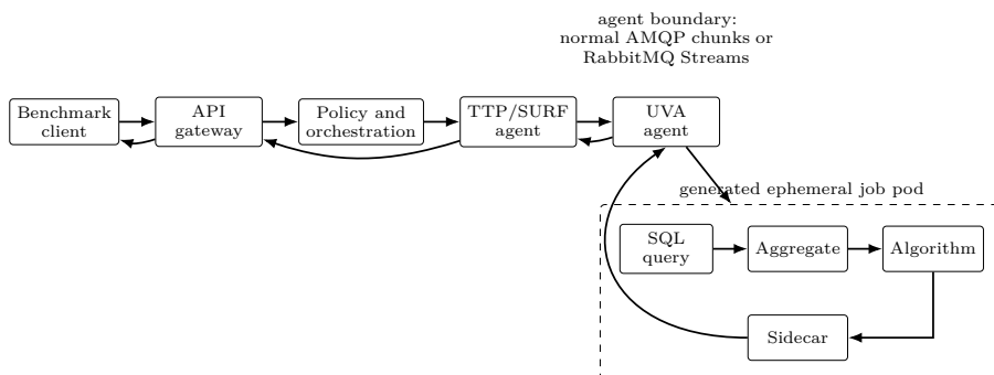
Figure 6.1: DYNAMOS bulk retrieval path used for RQ2. The implementation changes the bulk data path after policy approval. Chunking starts at the SQL query service and must be preserved through the generated job, agent path, and gateway response to avoid rebuilding one complete result table before the client sees progress.
