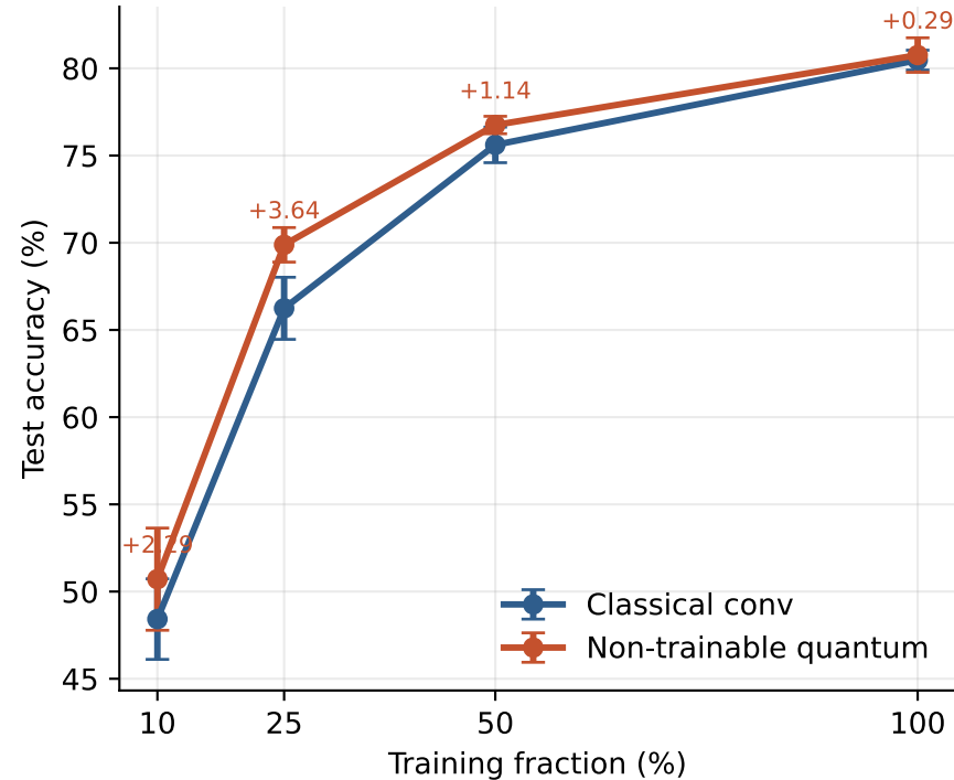
Current-local confirmation (3 seeds)
