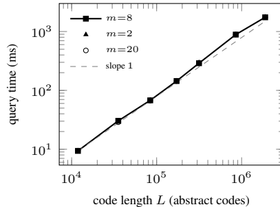
(b) query vs. |\text{code}| , m \in \{2, 8, 20\}
